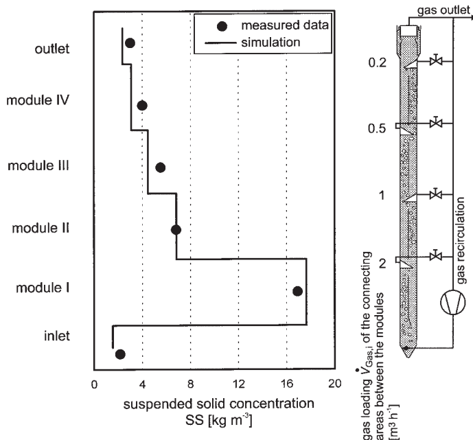
Fig. 6.30 Concentration of suspended solids as a function of reactor height in the 15 m 3 pilot scale BTR. \dot{V}_{\text{feed}} = 315 \text{ L h}^{-1} ; total gas production of the reactor 2.3 \text{ m}^3 \text{ h}^{-1} ; gas recirculated 1.8 \text{ m}^3 \text{ h}^{-1} ; \Delta\text{TOC} = 7.3 \text{ kg m}^{-3} ; gas loading V_{\text{gas},i} of the connecting areas between the modules as indicated.
