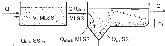
Fig. 3.26 Interaction between biological reactor and final clarifier.
