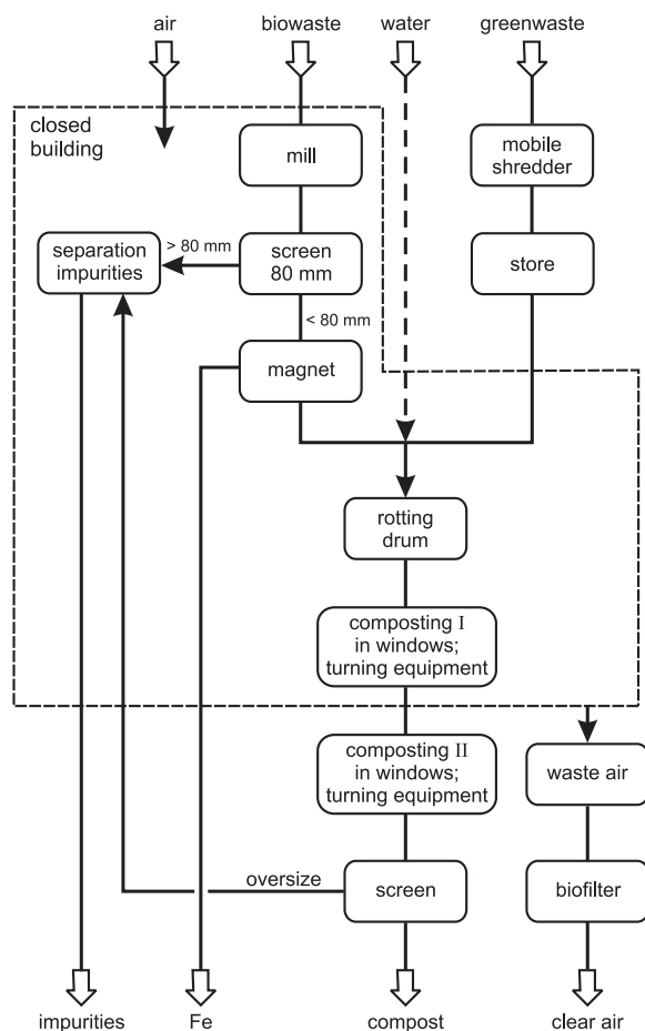
Fig. 13.14 Flow sheet of a composting plant with rotting drum in closed shed.
