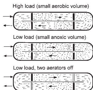
Fig. 3.19 Simultaneous nitrification and denitrification under different loading conditions.
