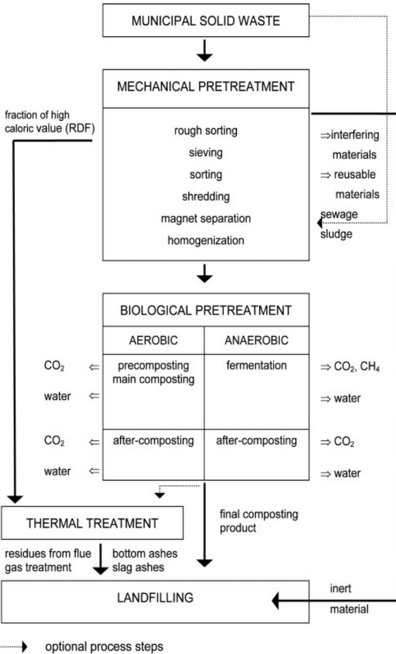
Fig. 15.3 Scheme of waste pretreatment before landfilling.
