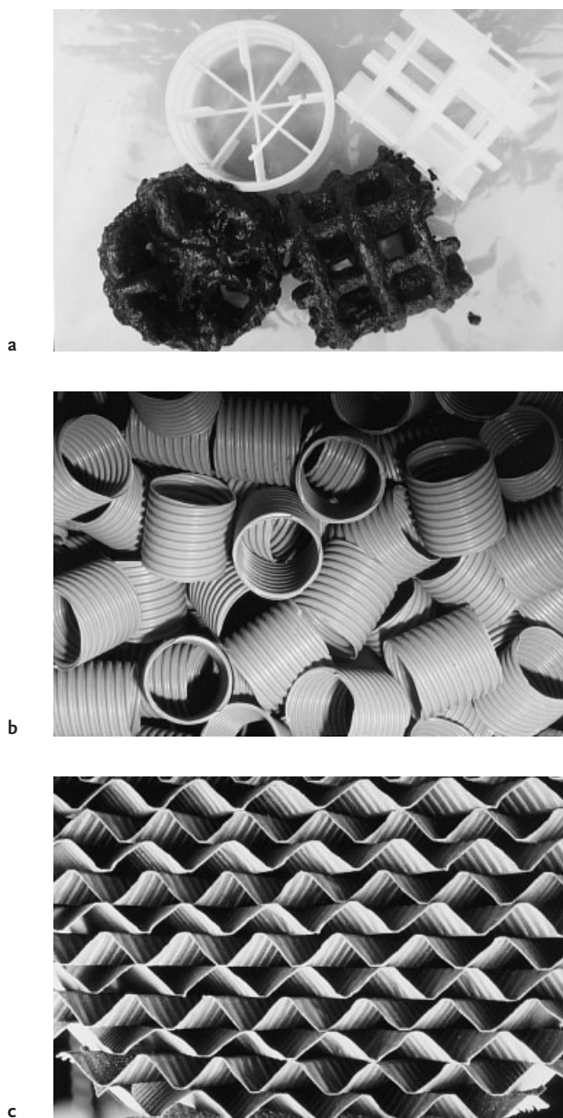
Fig. 5.4 Typical support materials for anaerobic stationary fixed-film reactors: a, Hiflow 90® (uncovered and biofilm-covered); b, Floccor R®; c, Plasdek C®. 10 (Weiland and Wulfert, 1986).
