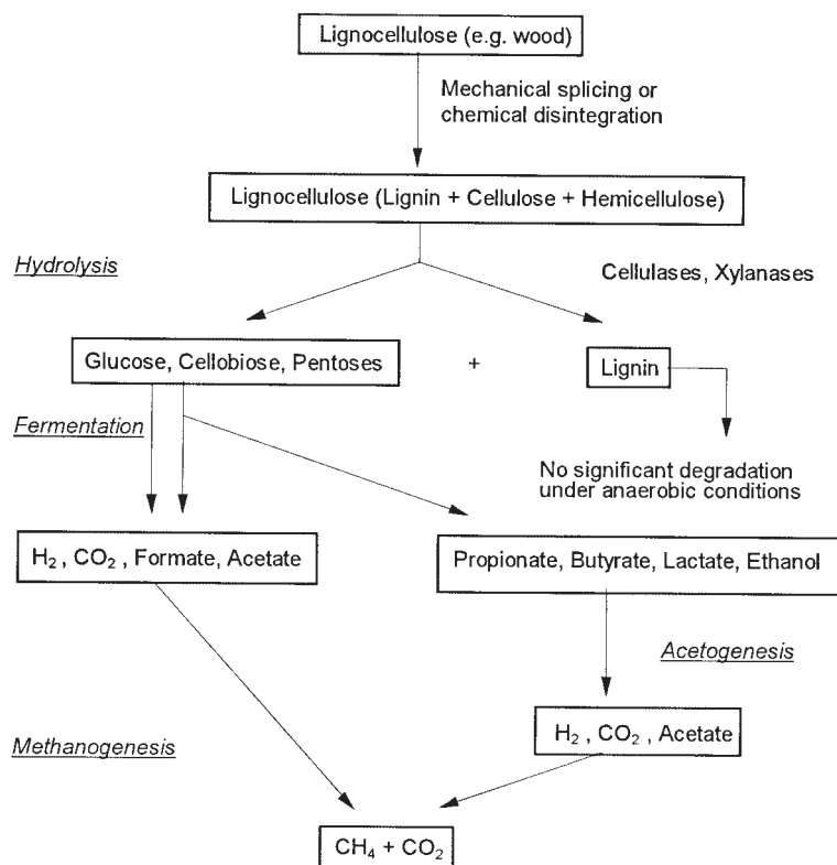
Fig. 1.3 Anaerobic degradation of lignocellulose and cellulose to methane and CO 2 (according to ATV, 1994).
