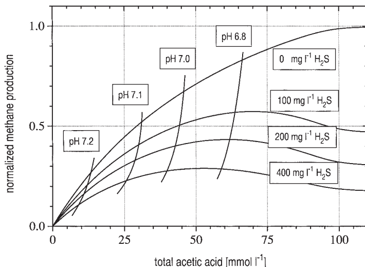
Fig. 6.17 Methane production as a function of the concentration of total acetic acid at different concentrations of total hydrogen sulfide ( c_{\text{HPro}} = 0 ).
