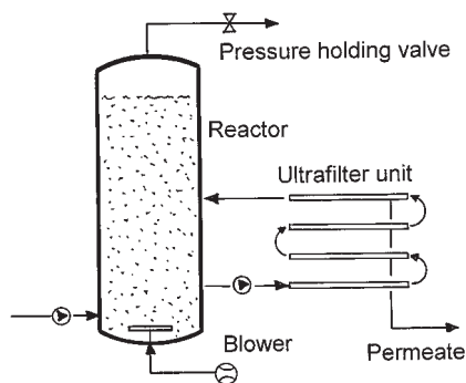
Fig. 3.7 Flow diagram of the Biomembrat process.
