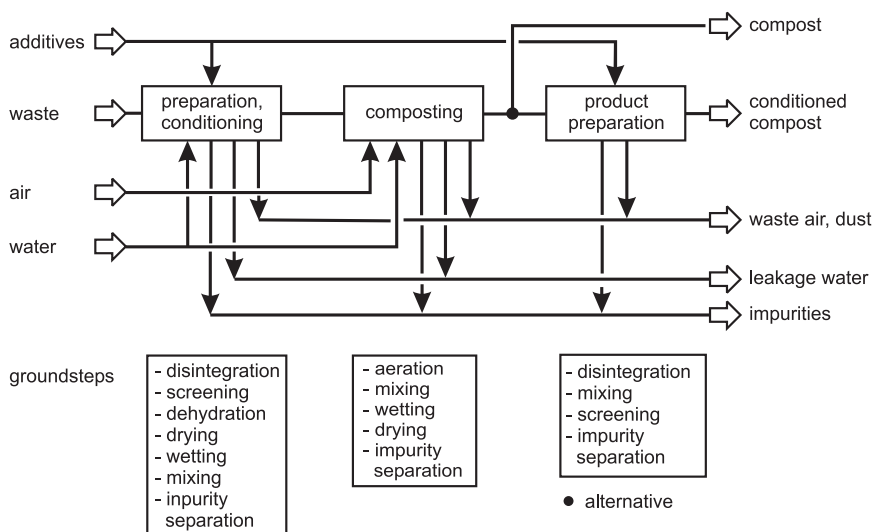
Fig. 13.5 Basic flow sheet of compost production.
