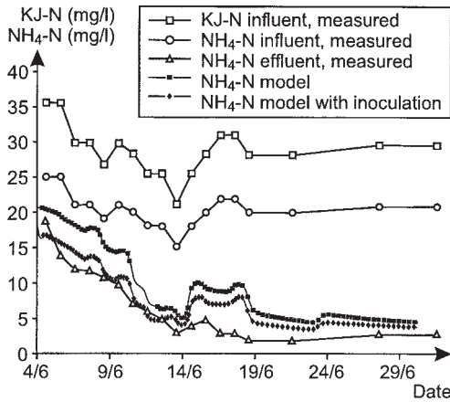
Fig. 4.5 Model calculation of startup of an activated sludge process with and without inoculation with nitrifying organisms (Finnson, 1994).
