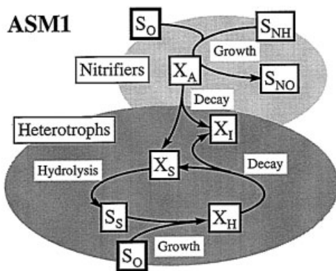
Fig. 4.1 Processes for heterotrophic and nitrifying bacteria in the Activated Sludge Model No. 1 (ASM1) (Gujer et al., 1999).
