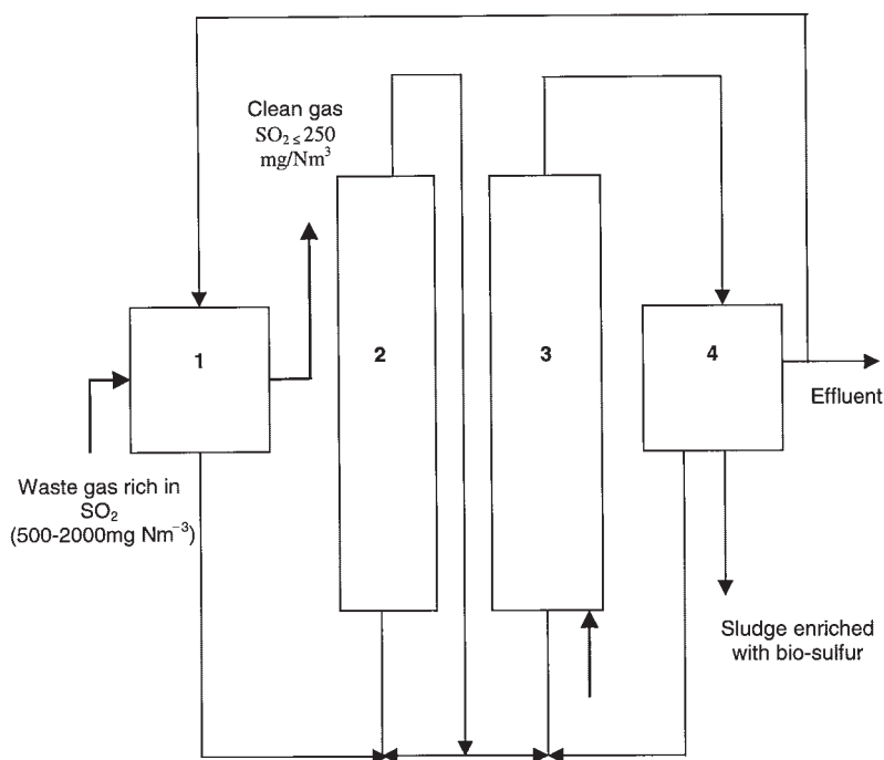
Fig. 17.4 Conversion of SO 2 by means of sulfate reduction and subsequent sulfide oxidation reactors to biologically formed elemental sulfur (after Grootaerd et al., 1977). 1: absorption of SO 2 gas; 2: sulfate reduction; 3: partial oxidation of hydrogen sulfide; 4: separation of sludge enriched with biosulfur.
