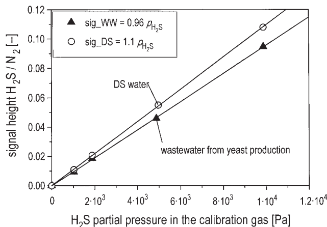
Fig. 6.5 Calibration of the silicon membrane probe coupled with a mass spectrometer measuring the concentration of dissolved \text{H}_2\text{S} in desalinated water (DS water) and in the wastewater of bakers' yeast production. The ordinate gives the value of the signal with reference to the \text{N}_2 signal of the carrier gas. The abscissa is the partial pressure of \text{H}_2\text{S} , with which the liquid is in equilibrium (after Polomski 1998).
