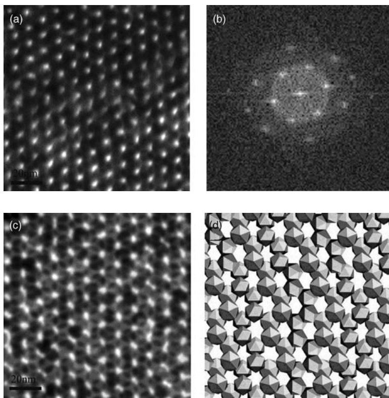
Figure 4.11 TEM images of Ag–Au alloy nanoparticles. (a) A multilayer; (b) The FFT pattern; (c) A two-layered sample; (d) The calculated model.
