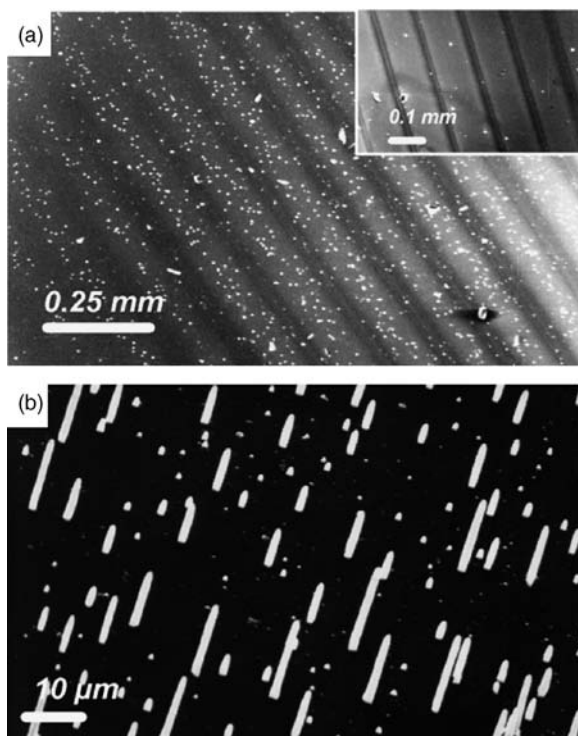
Figure 4.16 (a) Stripes of 9 nm \text{CoPt}_3 nanocrystals deposited in a magnetic field of 0.5 T applied parallel to a glass substrate; (b) Needles composed of 4.0 nm \text{CoPt}_3
