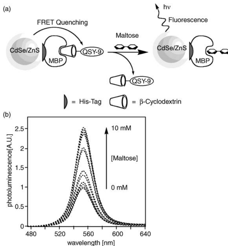
Figure 6.36 (a) Functionalized CdSe/ZnS QDs for the competitive assay of maltose using the maltose binding protein (MBP) as sensing material and \beta -cyclodextrin-QSY-9 dye conjugate \beta -CD-QSY-9 as FRET quencher; (b) Fluorescence changes of the MBP-functionalized QDs with increasing concentrations of maltose. (Reprinted by permission from Macmillan Publishers Ltd. Nature Materials Ref. [73]).
