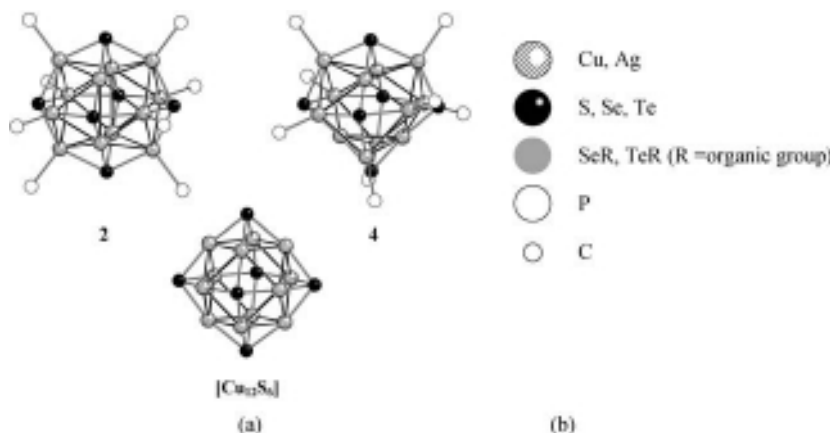
Figure 3.36 Molecular structures of [\text{Cu}_{12}\text{S}_6(\text{PEt}_2\text{Ph})_8] ( 2 ) and [\text{Cu}_{12}\text{S}_6(\text{PnPr}_3)_8] ( 4 ) (without organic groups) and of a calculated “naked” [\text{Cu}_{12}\text{S}_6] core. Cu: shaded spheres; S: black spheres; P: white spheres.
