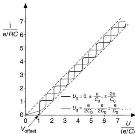
Figure 5.24 The dependence of the time-averaged current I versus U for an asymmetric single-electron transistor.
