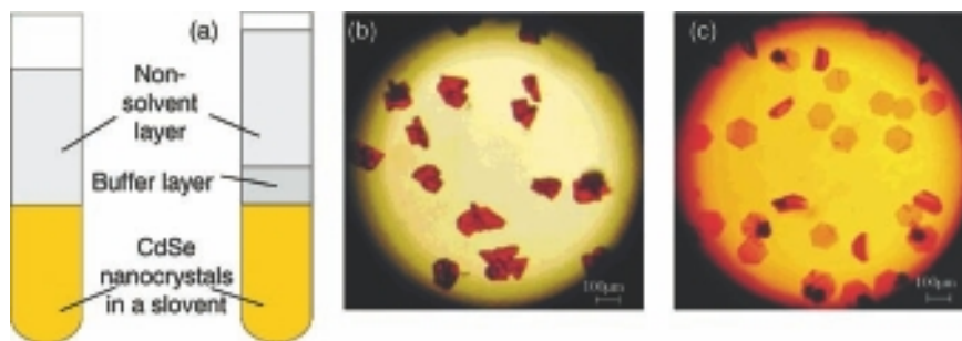
Figure 4.1 (a) Schematic illustration of superlattice formation from colloidal solutions of 3.5 nm CdSe nanocrystals in toluene; (b,c) Optical micrographs of the evolving nanocrystal superlattices after fast (b) and slow (c) nucleation. Reproduced with permission from Ref. [24].
