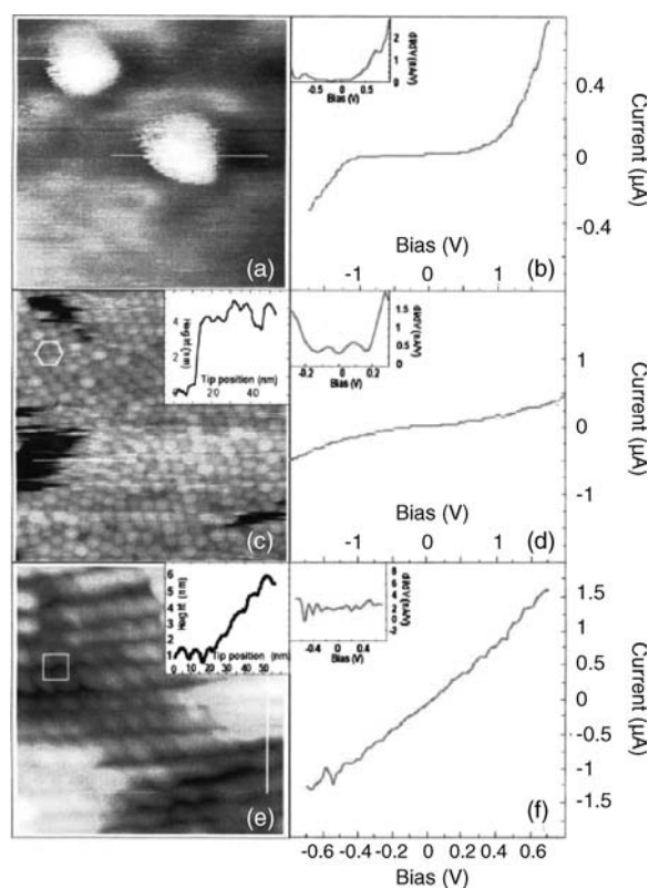
Figure 5.67 Left column: Constant-current mode STM image of isolated (a), self-organized in close-packed hexagonal network (c), and fcc structure (e) of silver nanoparticles deposited on an Au(111) substrate. Scan sizes: (a) 17.1 \times 17.1 \text{ nm}^2 , V_t = -1 \text{ V} , I_t = 1 \text{ nA} , (c) 136 \times 136 \text{ nm}^2 , V_t = 2.5 \text{ V} , I_t = 0.8 \text{ nA} , (e) 143 \times 143 \text{ nm}^2 , V_t = -2.2 \text{ V} , I_t = 0.72 \text{ nA} .
