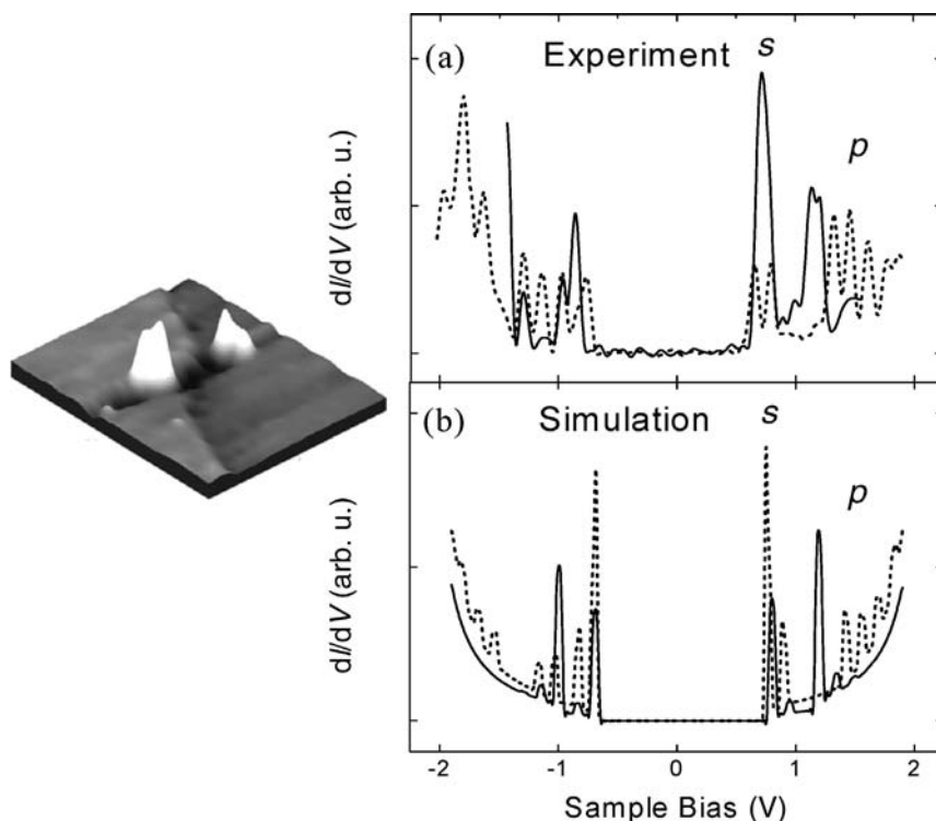
Figure 5.5 (a) Tunneling spectra measured on InAs QDs \sim 2 nm in radius. The solid curve was measured in the QD/HOPG geometry, and the dashed curve in the QD/DT/Au geometry; (b) Calculated spectra showing the effect of
