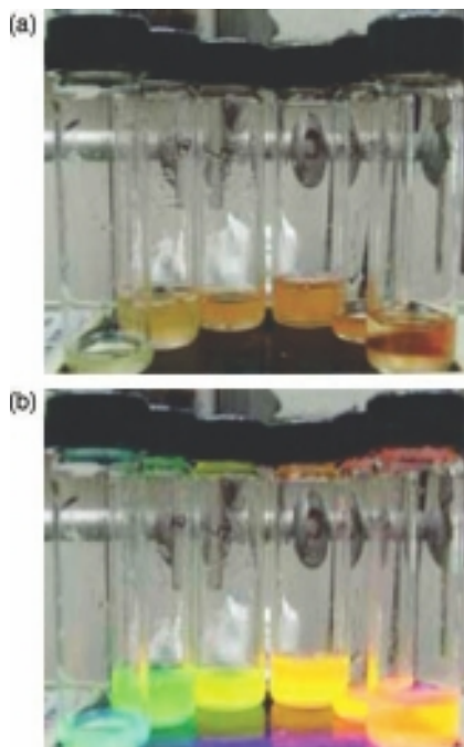
Figure 2.12 Colloidal CdSe QDs of different size dissolved in chloroform. The size of the QDs increases from the left to the right vial. (a) Photograph image
