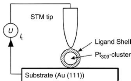
Figure 5.27 A single ligand-stabilized \text{Pt}_{309} -cluster between a STM tip and a Au(111) facet. The junction between the cluster and the substrate is built up by the ligand shell.
