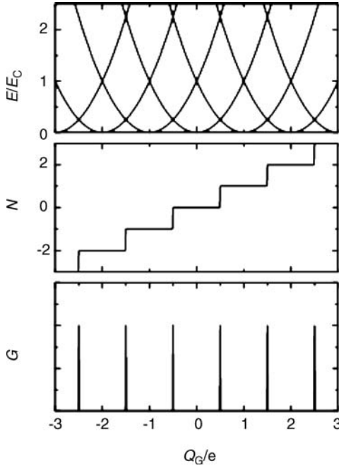
Figure 2.15 Schematic depiction of electrostatic energy E/E_C , occupation number N and conductance G of the single-electron transistor shown in Figure 2.14, as a function of the gate charge Q_G . The occupation of the single-electron transistor changes when the
