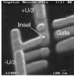
Figure 5.21 Scanning electron microscopy image of a single-electron transistor with source and drain ( +U/2 and -U/2 , respectively) feeding the central island (Insel), which is
