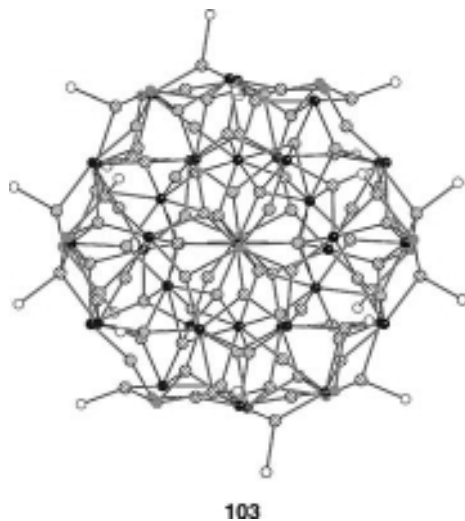
Figure 3.79 The core atoms in [Ag_{90}Se_{38}(SeiBu)_{14}(PEt_3)_{22}] ( 103 ). Ag: shaded spheres, Se: black spheres, SeR: gray spheres, P: white spheres.
