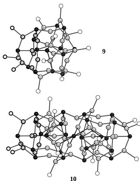
Figure 3.38 Molecular structures of [\text{Cu}_{28}\text{S}_{14}(\text{PtBu}_2\text{Me})_{12}] ( 9 ) and [\text{Cu}_{50}\text{S}_{25}(\text{PtBu}_2\text{Me})_{16}] ( 10 ) (without organic groups). Cu: shaded spheres; S: black spheres; P: white spheres. The atoms of topologically equal zones are highlighted in bold.
