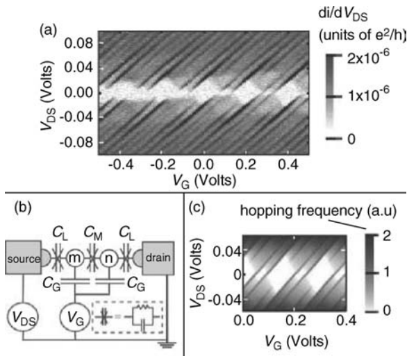
Figure 5.49 Experimental and predicted differential conductance plots of the double-island device of Figure 5.48. (a) Differential conductance measured at 4.2 K; four peaks are found per gate period. Above the threshold for the Coulomb blockade, the current can be described as linear with small oscillations superposed, which give the peaks in dI/dV_{DS} . The linear component corresponds to a resistance of \sim 20 \text{ G}\Omega ; (b) Electrical modeling of the device. The silicon substrate acts as a common gate electrode for both islands;
