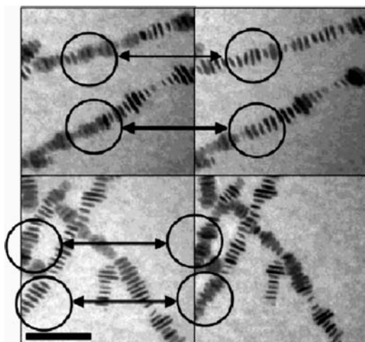
Figure 4.41 TEM image of stacked face-to-face hcp-Co nanodisks. The pictures on the left correspond to no tilt and those on the right the pictures on the right 25° tilt. The bar is 200 nm.
