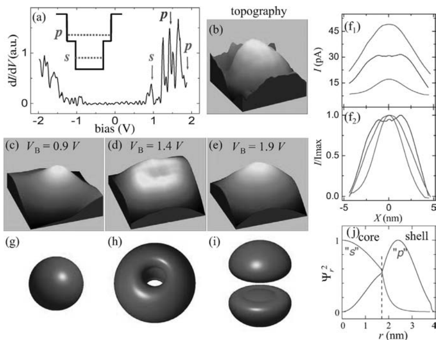
Figure 5.8 Wavefunction imaging and calculation for an InAs–ZnSe core–shell QD having a six ML shell. (a) A tunneling spectrum acquired for the nanocrystal; (b) 8 \times 8 \text{ nm}^2 topographic image taken at V_B = 2.1 \text{ V} and I_s = 0.1 \text{ nA} ; (c–e) Current images obtained simultaneously with the topographic scan at three different bias values denoted by arrows in panel (a); (f 1 ) Cross-sections taken along the diagonal of the current images at 0.9 \text{ V} (lower curve), 1.4 \text{ V} (middle curve) and 1.9 \text{ V} (upper
