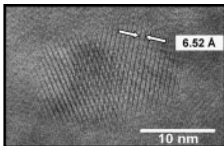
Figure 5.18 Section of a HR-TEM image of a microtome slice of a crystal of thermally treated [\text{Cu}_{70}\text{Se}_{35}(\text{PEt}_2\text{Ph})_{23}] (4).
