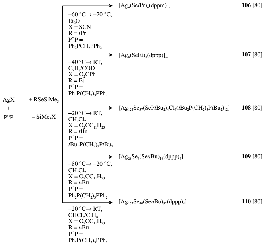
Scheme 3.14 The synthesis of selenido-selenolato-bridged silver clusters with bidentate phosphine ligands.
