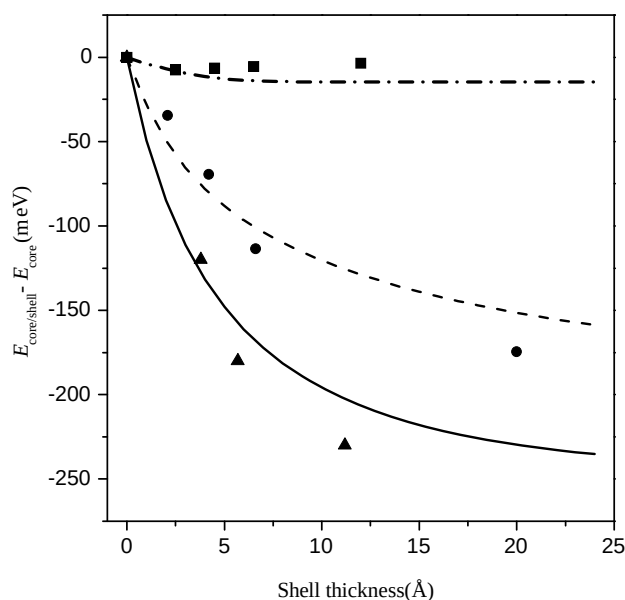
Figure 3.34 Experimental and calculated shifts of the band gap energy in various core–shells versus the shell thickness. InAs–ZnS core–shells: experimental data = squares, calculated shift of gap = dot-
