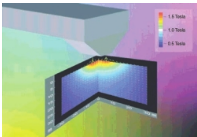
Figure 3.151 Dependence of the magnetic flux density on the distance to pole shoe with the electromagnet. Reproduced with permission from Ref. [218]; © 2000, American Association for Cancer Research.
