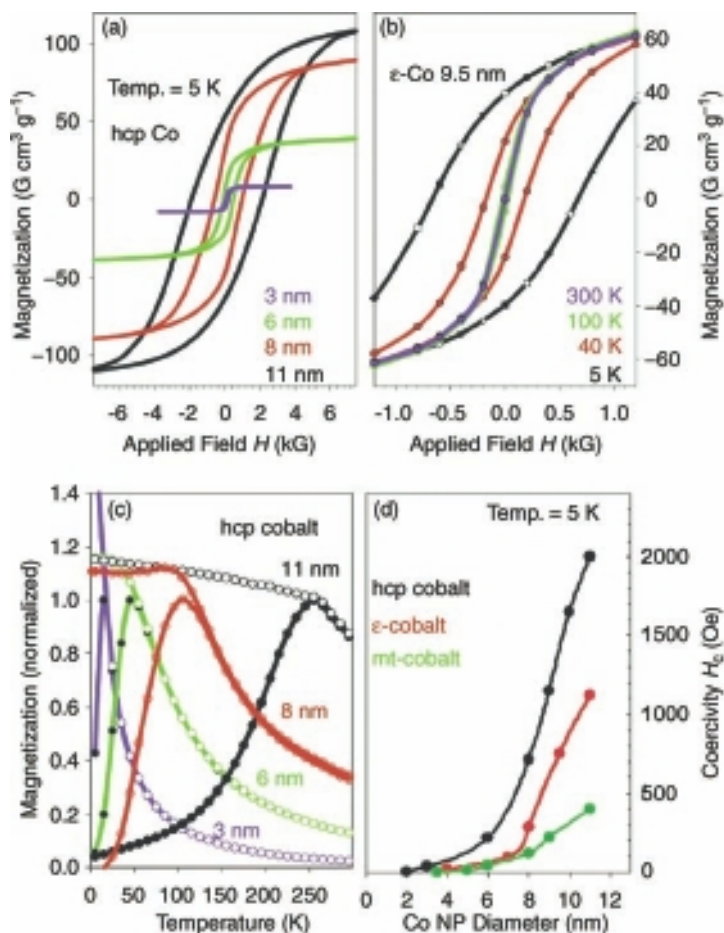
Figure 3.144 (a) Magnetization versus applied-field hysteresis loops at 5 K for 3, 6, 8, and 11 nm hcp cobalt nanocrystals; (b) Comparison of the hysteresis loops for 9.5 nm \epsilon -Co nanocrystals measured at 5, 40, 100, and 300 K; (c) A series of zero-field-cooled (ZFC) and field-cooled (FC) magnetization scans
