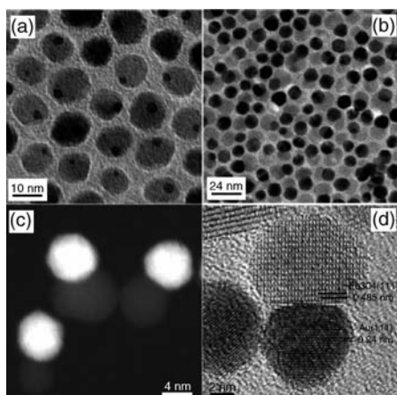
Figure 3.134 TEM images of (a) 3–14 nm and (b) 8–14 nm Au-Fe 3 O 4 nanodumbbells; (c) High-angle annular dark-field scanning electron micrograph of the 8–9 nm Au-Fe 3 O 4 particles; (D) HR-TEM image of a 8–12 nm Au-Fe 3 O 4 nanodumbbell. Reproduced with permission from Ref. [139]; © 2005, American Chemical Society.
