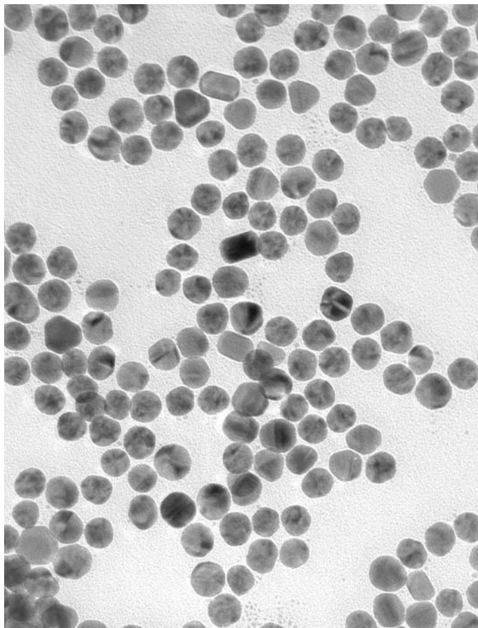
Figure 3.104 TEM image of monodispersed 18 nm gold particles, prepared by citrate reduction of \text{HAuCl}_4 .
