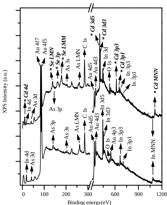
Figure 3.29 XPS survey spectrum for InAs cores with radius of 1.7 nm (lower trace), and for InAs–CdSe core-shells with shell thickness of three monolayers (top trace). The assignment of
