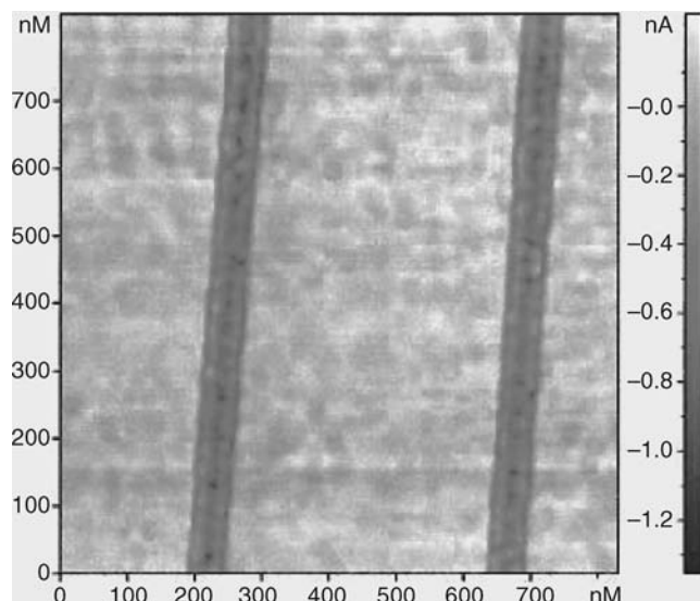
Figure 4.44 Magnified pieces of \text{Au}_{55} cluster-decorated lines of Figure 4.43, indicating two rows of clusters per line.
