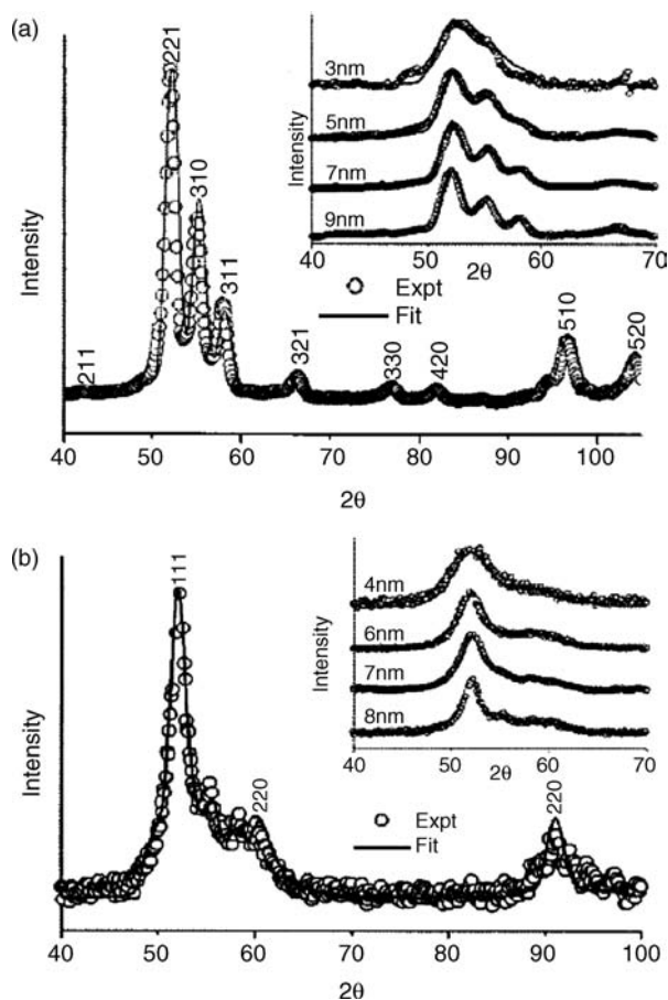
Figure 3.115 Powder XRD patterns for cobalt nanoparticles (circles) and their corresponding simulations (solid lines) using atomic-level models of the particles. (a) \epsilon -Co; (b) multiply-
