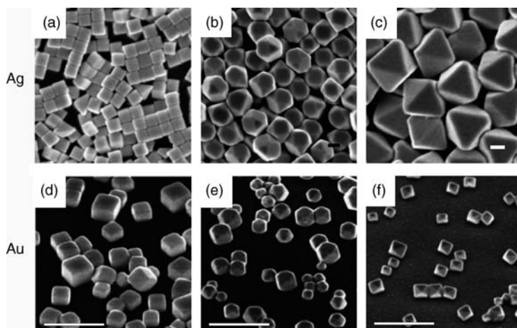
Figure 3.112 Silver cubes (a), cubo-octahedra (b), and octahedra (c). (Scale bar = 100 nm); (d–f) The same shapes, but with gold nanoparticles (scale bar = 1 \mu\text{m} ).
