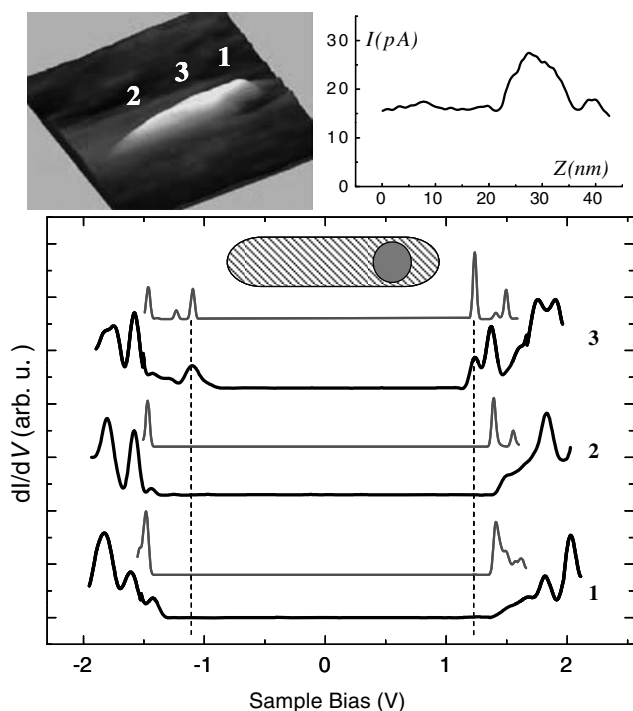
Figure 5.10 Three tunneling spectra (black curves) acquired on a CdSe/CdS nanocrystal at locations marked on the topographic image shown to the top-left. The corresponding theoretical curves are drawn above the
