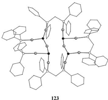
Figure 3.102 The molecular structure of the cationic framework in [\text{Au}_{10}\text{Se}_4(\text{Ph}_2\text{PCH}_2\text{PPh}_2)_4]\text{Br}_2 ( 123 ) (without H atoms). Au: shaded spheres; Se: black spheres; P: white spheres; C: wire representation.
