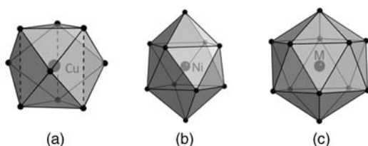
Figure 3.7 Representative Zintl ions with one endohedral metal atom. (a) [\text{Cu}@\text{E}_9]^{3-} ( \text{E} = \text{Sn} , \text{Pb} ) [68]; (b) [\text{Ni}@\text{Pb}_{10}]^{2-} [69]; (c) [\text{M}@\text{Pb}_{12}]^{2-} ( \text{M} = \text{Ni} , \text{Pd} , \text{Pt} ) [71, 72] and [\text{Ir}@\text{Sn}_{12}]^{3-} [58].
