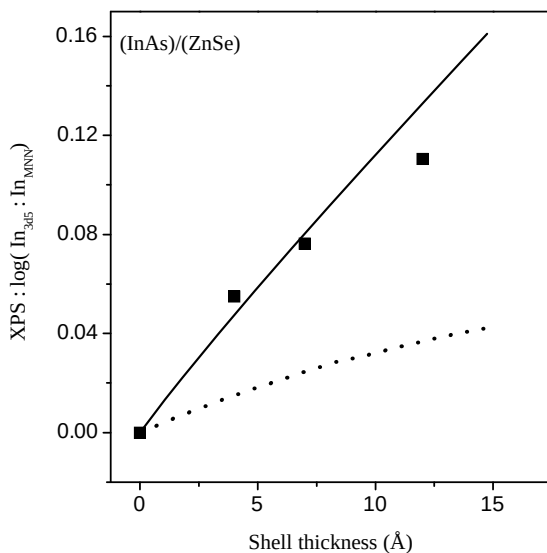
Figure 3.30 Summary of high-resolution XPS data for InAs–ZnSe. The log of the ratio of the intensities of the \text{In}_{3d5} to the \text{In}_{\text{MNN}} is shown, versus the shell thickness. The ratio is normalized to the ratio in the cores.
