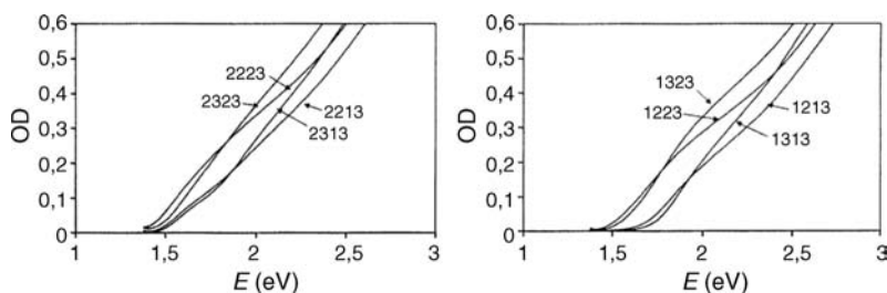
Figure 3.20 Absorption spectra of eight different double-well nanoheterostructures. In CdS nanocrystals, two wells of HgS are embedded, well thickness and well separations are varied (for details of nomenclature, see the text). From Ref. [308].
