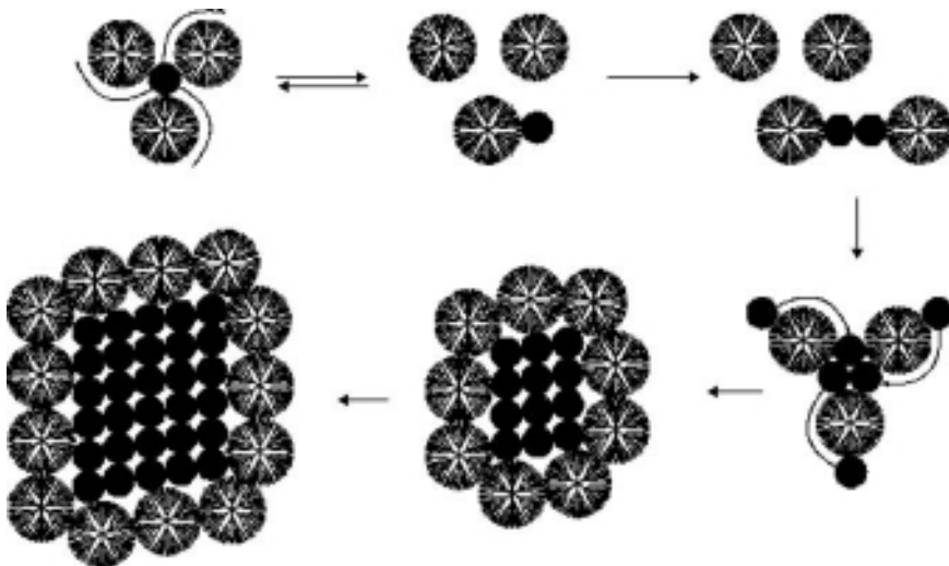
Figure 4.8 Schematic representation of the formation of \text{Au}_{55} microcrystals inside a matrix of G4-SH dendrimers.
