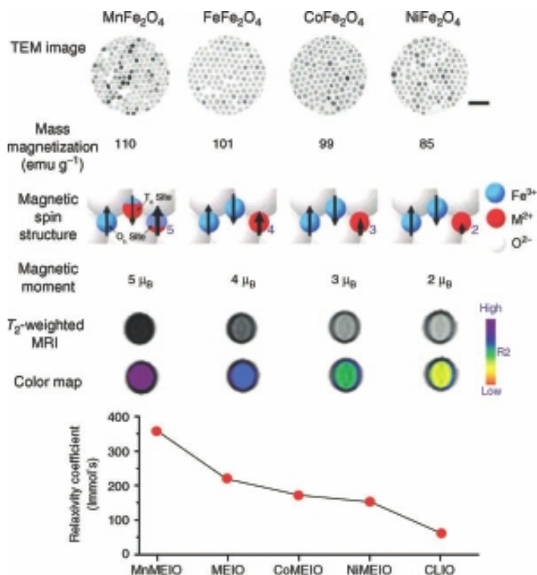
Figure 3.155 Transverse relaxivity of various uniformly sized spinel ferrite nanoparticles with respect to composition. r_2 correlates strongly with the saturation magnetization M_s [129]. Reproduced with permission from Ref. [129]; © 2007, Nature Publishing Group.
