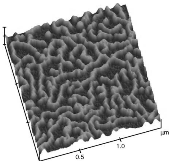
Figure 4.23 AFM image of \text{Au}_{55}(\text{PPh}_3)_{12}\text{Cl}_6 clusters decorating chains of PVP, forming a 2-D network.
