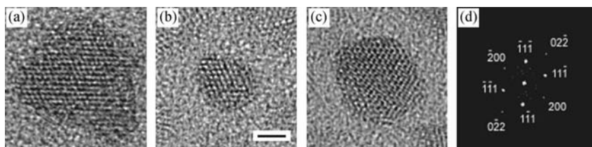
Figure 3.31 HR-TEM images of (a) InAs–InP core–shell (core radius 1.7 nm, shell thickness 2.5 nm), (b) InAs core (core radius 1.7 nm), and (c) InAs–CdSe core–shell (core radius 1.7 nm, shell thickness 1.5 nm). The scale bar is 2 nm.
