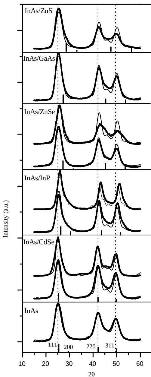
Figure 3.33 X-ray diffraction patterns for InAs cores and various core shells. The experimental curves (filled circles), are compared with the simulated curves (thin solid lines). See text and Table 1 for details of the simulated structures. The markers at the bottom of each frame
