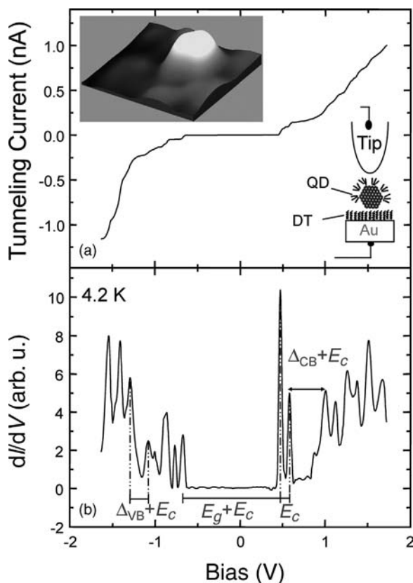
Figure 5.2 STM measurements on single InAs nanocrystal 3.2 nm in radius, acquired at 4.2 K. The QDs are linked to the gold substrate by dithiol (DT) molecules, as shown schematically in the right inset. The left inset presents a 10 \times 10 nm STM topographic image of the QD. The tunneling I – V characteristic is presented in
