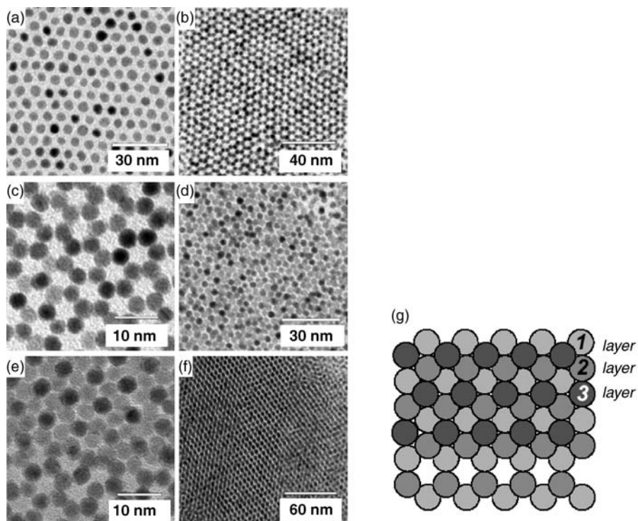
Figure 4.19 TEM images. (a) A monolayer of 4.8 nm CoPt 3 nanoparticles; (b,c) Two layers of 3.6 and 4.0 nm CoPt 3 nanoparticles; (d) Three layers of 3.6 nm CoPt 3 nanoparticles; (e) Three layers of 4.0 nm CoPt 3 nanoparticles; (f) More
