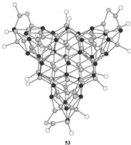
Figure 3.64 Molecular structure of [\text{Cu}_{73}\text{Se}_{35}(\text{SePh})_3(\text{PiPr}_3)_2] ( 53 ) (without organic groups). Cu: shaded spheres; Se: black spheres; SeR: gray spheres; P: white spheres.
