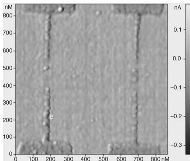
Figure 4.46 Optimized pattern of ideal 1-D cluster wires and single clusters in predefined intrawire gaps.
