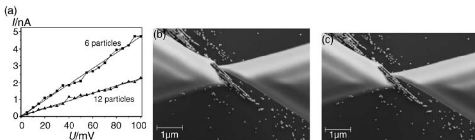
Figure 5.55 (a) I(V) characteristics of O_3 -cleaned samples; (b,c) Corresponding SEM images of the electrical transport measurements. Reproduced with kind permission from Ref. [68]; © 2008, American Scientific Publishers.
