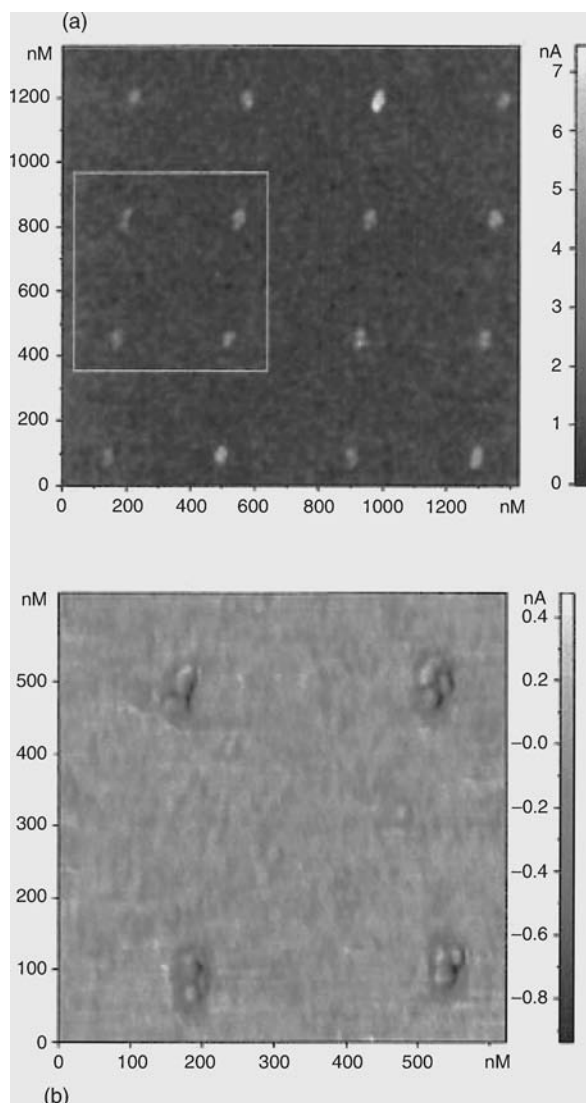
Figure 4.45 AFM images of a regular arrangement of dots of Au 55 clusters, each dot consisting of two to three clusters.
