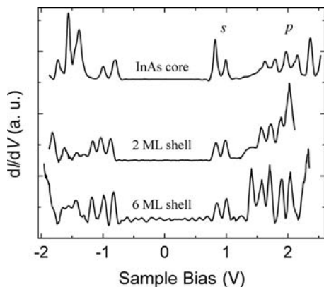
Figure 5.6 Tunneling conductance spectra of an InAs core QD and two core–shell nanocrystals with two and six monolayer (ML) shells with nominal core radii \sim 1.7 nm. The spectra were offset along the V direction to center the observed zero current gaps at zero bias.
