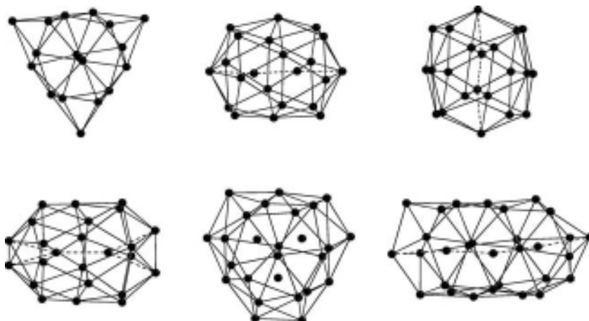
Figure 3.46 Selenium substructures in 22–27 (from top left to bottom right). The drawn Se–Se contacts do not represent bonding interactions, but rather illustrate the geometries of the polyhedra.
