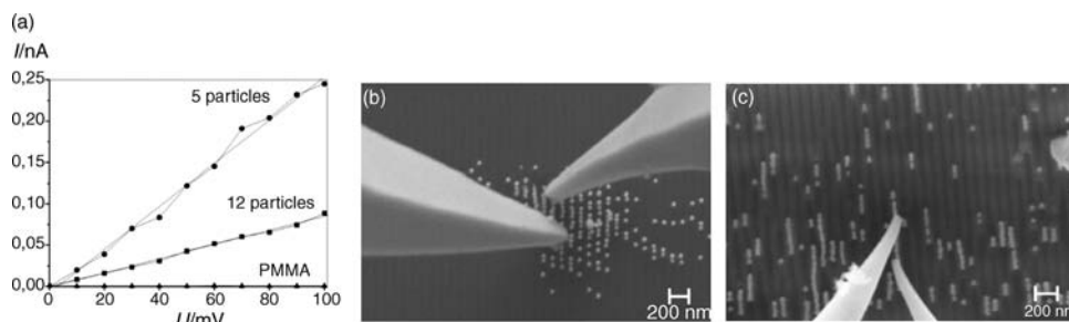
Figure 5.54 (a) I(V) characteristics of as-prepared gold nanoparticle chains with different numbers of particles and a reference measurement on the PMMA surface; (b,c) Corresponding SEM images of the
