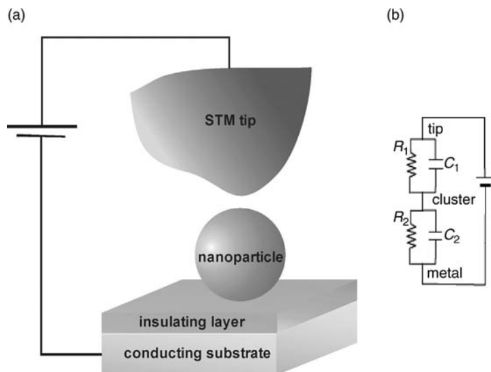
Figure 5.25 (a) General scheme of the STM configuration for the investigation of SET on individual metal nanoparticles; (b) Corresponding electronic circuit
