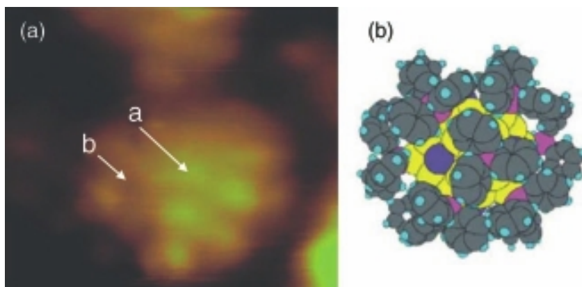
Figure 5.29 (a) STM image of a single \text{Au}_{55}[\text{P}(\text{C}_6\text{H}_5)_3]_{12}\text{Cl}_6 cluster on a \text{Au}(111) surface at 7 K, obtained at a bias of 2 V and a current of 100 pA using a Pt–Ir tip. Image size: 3.3 \times 2.9 nm; (b) Space-filling model of the cluster compound: cubo-octahedral core with 55 Au atoms (yellow), 12 \text{P}(\text{C}_6\text{H}_5)_3 molecules (with P pink, C gray and H blue) bound to the
