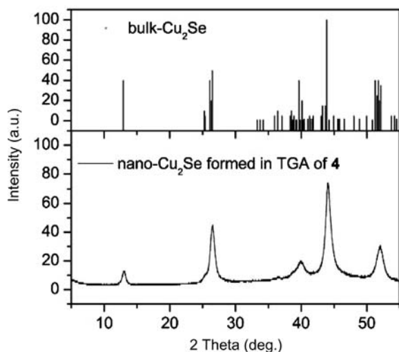
Figure 5.17 X-ray powder diffraction pattern of the black residue of the thermogravimetric analysis of [\text{Cu}_{70}\text{Se}_{35}(\text{PEt}_2\text{Ph})_{23}] ( 4 ) in vacuum (lower graph) and of monoclinic \alpha\text{-Cu}_2\text{Se} [115] (upper graph).
