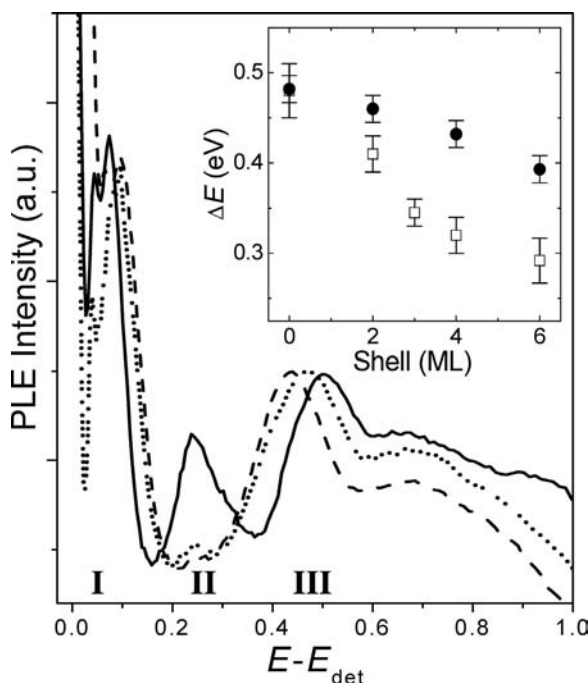
Figure 5.7 PLE spectra, normalized to peak III, for InAs cores (solid line) and InAs-ZnSe core-shell nanocrystals of four-ML (dotted line) and six-ML (dashed line) shells, with the zero of the energy scale taken at the detection window (970 nm). The inset depicts the dependence on
