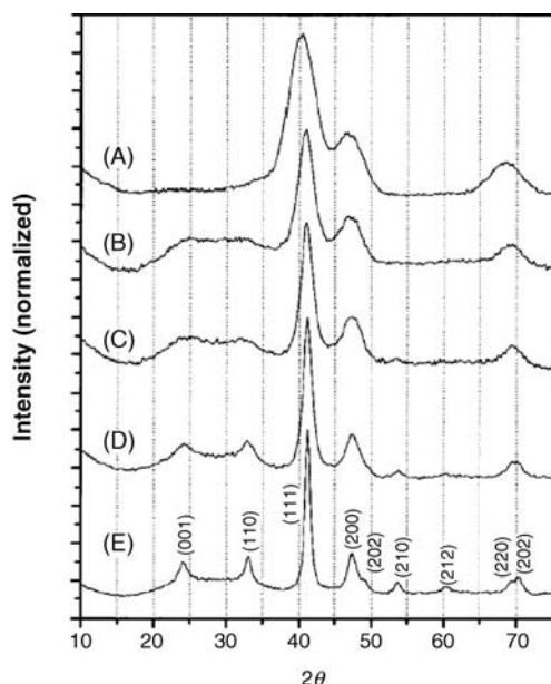
Figure 3.129 XRD patterns (A) of as-synthesized 4 nm \text{Fe}_{52}\text{Pt}_{48} particle assemblies and a series of similar assemblies annealed under atmospheric \text{N}_2 gas for 30 min at temperatures of (B) 450 °C, (C) 500 °C, (D) 550 °C, and (E) 600 °C.
