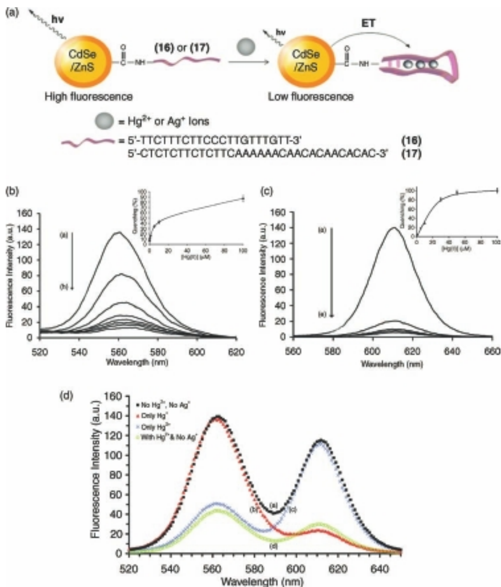
Figure 6.9 (a) Optical analysis of \text{Hg}^{2+}/\text{Ag}^{+} ions by nucleic acid modified QDs; (b) Time-dependent luminescence spectra of 16-QD 560 upon interaction with 1 \times 10^{-4} M \text{Hg}^{2+} . Inset: Calibration curve for various concentrations of \text{Hg}^{2+} ; (c) Time-dependent luminescence spectra of 17-QD 620 upon interaction with 5 \times 10^{-5} M \text{Ag}^{+} . Inset: Calibration curve for
