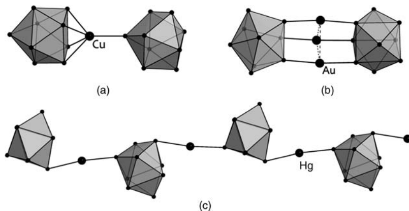
Figure 3.6 Zintl ions with ligand-free d-block metal atoms. (a) [(\eta^4\text{-Ge}_9)\text{Cu}(\eta^1\text{-Ge}_9)]^{7-} [59]; (b) [\text{Ge}_9\text{Au}_3\text{Ge}_9]^{5-} [65]; (c) {}^\infty[(\text{Hg Ge}_9)^{2-}] [61].
