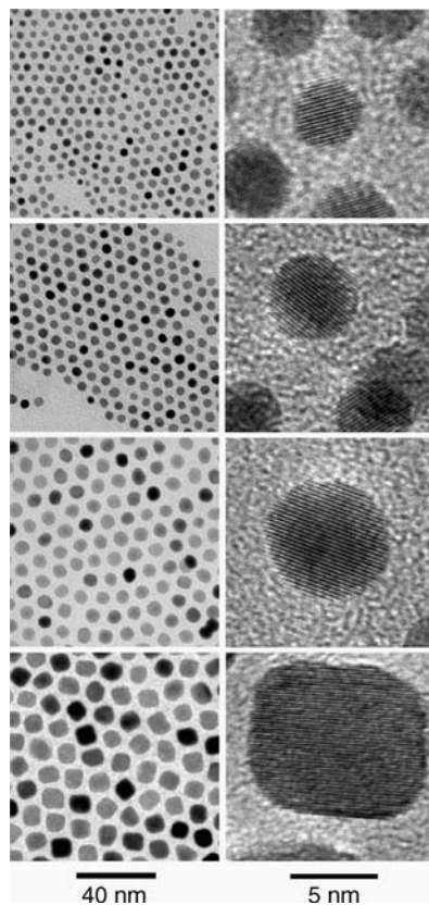
Figure 3.124 TEM and HR-TEM images showing the effect of the reaction temperature on the mean size and size distribution of 3.7 nm, 4.9 nm, 6.3 nm and 9.3 nm \text{CoPt}_3 nanocrystals prepared at 220, 200, 170 and
