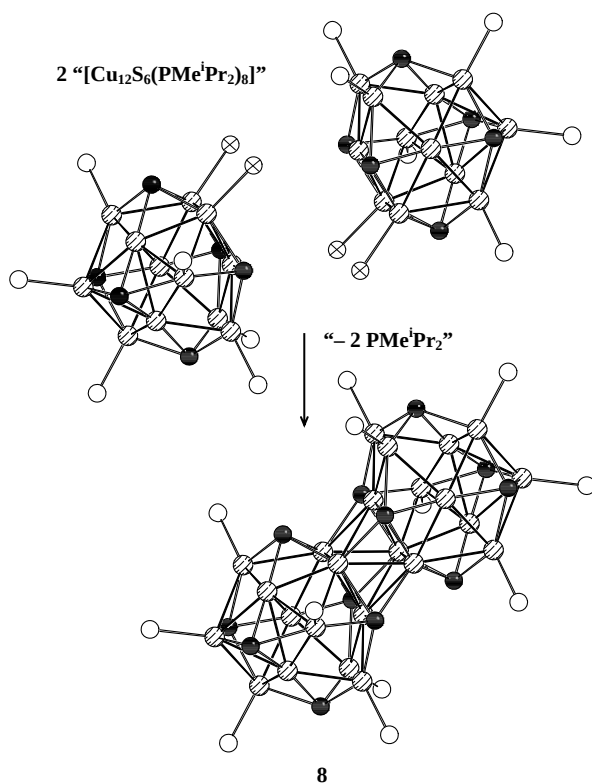
Figure 3.37 Formal dimerization–condensation reaction of two hypothetical clusters “ [\text{Cu}_{12}\text{S}_6(\text{Me}^i\text{Pr}_2)_8] ,” resulting in the molecular structure of [\text{Cu}_{24}\text{S}_{12}(\text{PMeiPr}_2)_{12}] ( 8 ) (without organic groups). Cu: shaded spheres;
