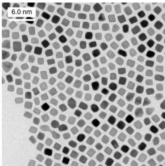
Figure 3.125 TEM overview image of faceted CoPt 3 nanocrystals prepared at 145 °C.
