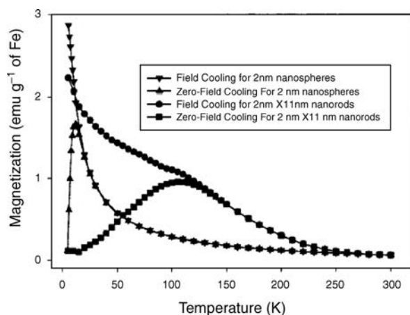
Figure 3.145 Zero-field-cooled (ZFC) and field-cooled (FC) magnetization scans for the 2 nm spherical iron nanoparticles and the 2 nm \times 11 nm iron nanorods at the applied magnetic field of 100 Oe. Reproduced with permission from Ref. [82]; © 2000, American Chemical Society.
