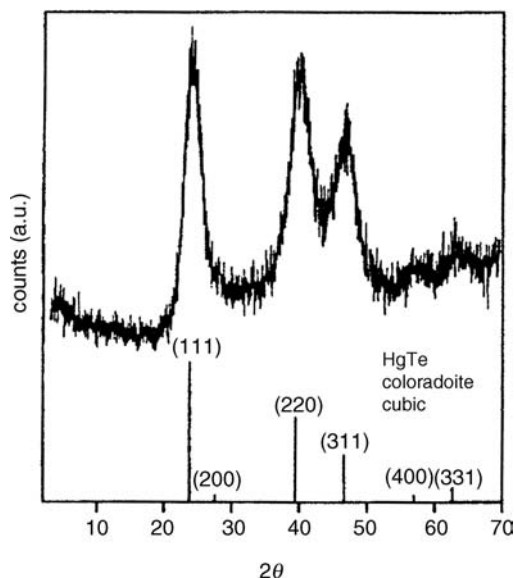
Figure 3.14 Powder X-ray diffractogram of HgTe nanocrystals (“thiol synthesis”) with corresponding bulk values given as a line spectrum. From Ref. [37].
