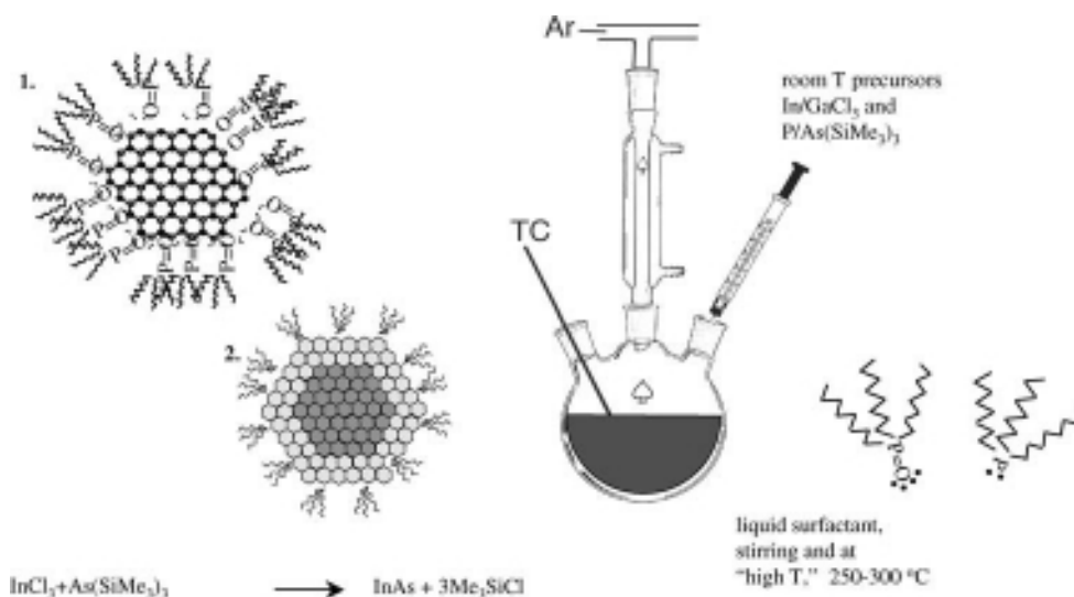
Figure 3.21 Schematic reaction set-up and reaction scheme for III–V semiconductor nanocrystals, either for cores coated by organic ligands (1), or for core–shell nanocrystals (2).
