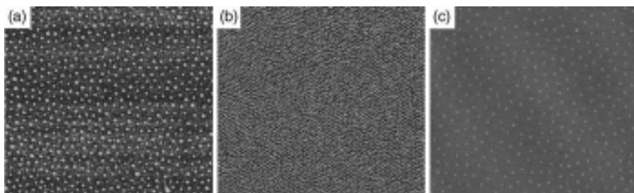
Figure 4.32 TEM images of gold nanoparticles of various sizes generated in micelles of different sizes and by different loading ratios. (a) 6 nm, (b) 4 nm, (c) 2.5 nm.
