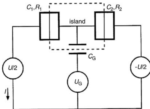
Figure 5.22 Circuit equivalent of a simple single-electron transistor, consisting of a two-junction arrangement and a gate electrode coupled capacitively to the central island. The
