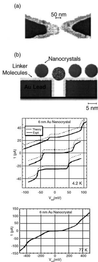
Figure 5.34 (a) Field-emission scanning electron microscopy image of a lead structure before the nanoparticles are introduced. The light gray region is formed by the angle evaporation, and is \sim 10 nm thick. The darker region is from a normal angle evaporation and is \sim 70 nm thick; (b) Schematic cross-section of nanoparticles bound via a bifunctional linker molecule to the leads. Transport between the leads occurs through the mottled nanoparticle bridging the gap; (c) I(V_{sd}) characteristics of a 5.8 nm-diameter Au nanoparticle measured at
