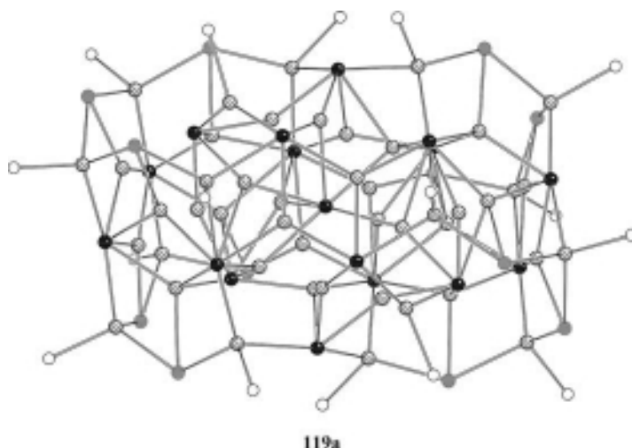
Figure 3.98 The molecular structure of [\text{Ag}_{46}(\text{Temes})_{12}\text{Te}_{17}(\text{PEt}_3)_{16}] ( 119a ) (without organic groups). Ag: shaded spheres; Te: black spheres; TeR: gray spheres; P: white spheres.
