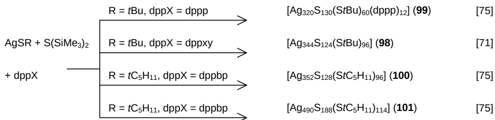
Scheme 3.12 Synthesis of various metal-rich, sulfur-bridged silver clusters by reactions of silver thiolates \text{S}(\text{SiMe}_3)_2 in the presence of bidentate phosphanes.
