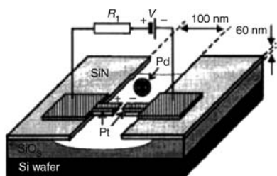
Figure 5.35 Schematic representation of the set-up for single particle measurements. Pt denotes two freestanding Pt electrodes (dashed region). A ligand-stabilized Pd cluster is
