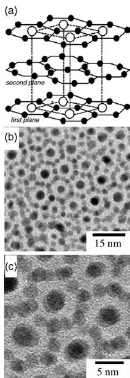
Figure 4.18 (a) Schematic view of an intermetallic compound \text{CaCu}_5 ; (b,c) TEM images illustrating an \text{AB}_5 -type superstructure formed by \text{CoPt}_3 nanocrystals with bimodal size distribution. Reproduced with permission from Ref. [26]; © 2002, American Chemical Society.
