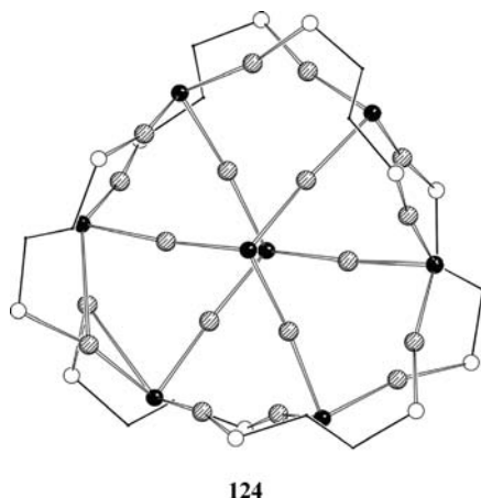
Figure 3.103 A projection of the molecular structure of [\text{Au}_{18}\text{Se}_8(\text{Ph}_2\text{P}(\text{CH}_2)_2\text{PPh}_2)_4]^{2+} ( 124 ) (H atoms and phenyl rings omitted for clarity). Au: shaded spheres; Se: black spheres; P: white spheres; C: wire representation.
