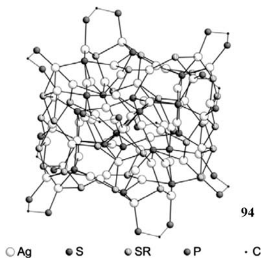
Figure 3.73 The molecular structure of [\text{Ag}_{70}\text{S}_{20}(\text{SPh})_{28}(\text{dppm})_{20}]^{2+} in 94 .
