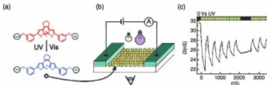
Figure 5.62 (a) Scheme of the switching molecule, a dithiolated diarylethene. Top: closed form (“on” state). Bottom: open form (“off” state); (b) Scheme of the measuring set-up for the light-induced conductance switching;
