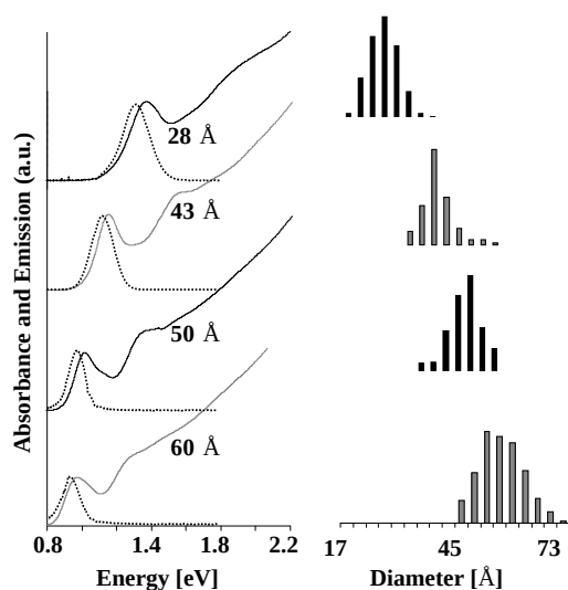
Figure 3.25 The right-hand panel shows the distribution of diameters for four InAs nanocrystal samples obtained from HR-TEM measurements. The left panel displays the room-temperature absorption (solid lines), and emission spectra (dashed lines) for the corresponding samples. The mean diameter for each sample is noted. Reproduced from Ref. [15].
