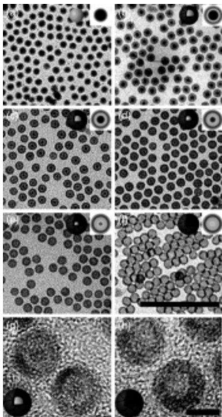
Figure 3.137 Hollow iron–iron oxide nanocrystals formed by the nano-Kirkendall effect. TEM images of iron–iron oxide nanoparticles exposed to dry 20% oxygen. (a) <1 min at room temperature; (b) 1 h at 80 °C; (c) 12 h at 80 °C; (d) 5 min at 150 °C; (e) 1 h at 150 °C; (f) 1 h at 350 °C on a substrate; (g,h) High-resolution of partial and fully oxidized iron nanoparticles. The low- and high-resolution scale bars correspond to 100 and 6 nm,
