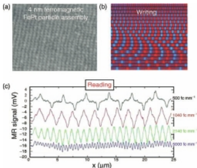
Figure 3.146 Magneto-resistive (MR) read-back signals from written bit transitions in a 120 nm-thick assembly of 4 nm-diameter \text{Fe}_{48}\text{Pt}_{52} nanocrystals. The individual line scans reveal magnetization reversal transitions at linear densities of 500, 1040, 2140, and 5000 flux changes per millimeter ( \text{fc mm}^{-1} ) [86]. Courtesy of C. B. Murray.
