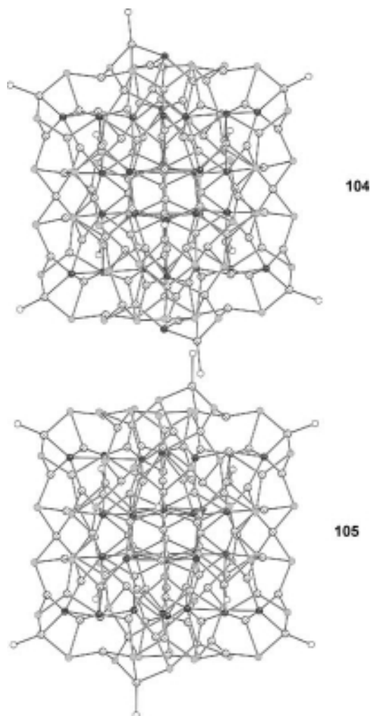
Figure 3.81 The core structures in [\text{Ag}_{114}\text{Se}_{34}(\text{SenBu})_{46}(\text{PtBu}_3)_{14}] ( 104 ) (top) and [\text{Ag}_{112}\text{Se}_{32}(\text{SenBu})_{48}(\text{PtBu}_3)_{12}] ( 105 ) (bottom). Ag: shaded spheres, Se: black spheres, SeR: gray spheres, P: white spheres.
