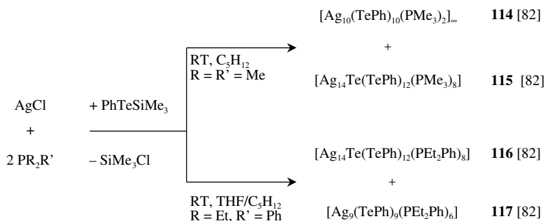
Scheme 3.16 The synthesis of telluride–telluroato-bridged silver clusters with monodentate phosphine ligands.
