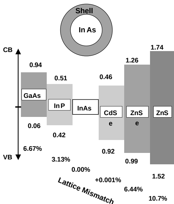
Figure 3.26 Summary of the band offsets (in eV) and lattice mismatch (in %) between the core InAs and the III–V semiconductor shells (left side), and II–VI semiconductor shells (right side) grown in these studies. CB = conduction band; VB = valence band. Reproduced from Ref. [7].
