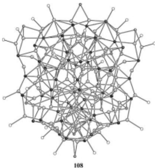
Figure 3.86 A projection of the molecular structure of [\text{Ag}_{124}\text{Se}_{57}(\text{SePtBu}_2)_4\text{Cl}_6(\text{tBu}_2\text{P}(\text{CH}_2)_3\text{PtBu}_2)_{12}] ( 108 ) (without organic groups). Ag: shaded spheres; Se: black spheres; SeR: gray spheres; P: white spheres.
