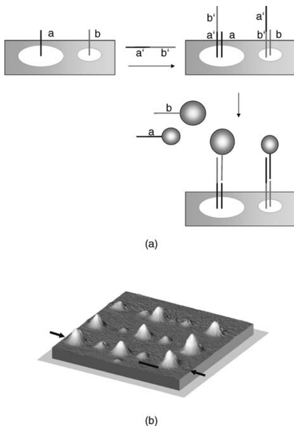
Figure 4.36 (a) Schematic illustration of the formation of gold nanostructures via complementary oligonucleotides; (b) AFM image of as-prepared patterns consisting of gold nanoparticles of different sizes.
