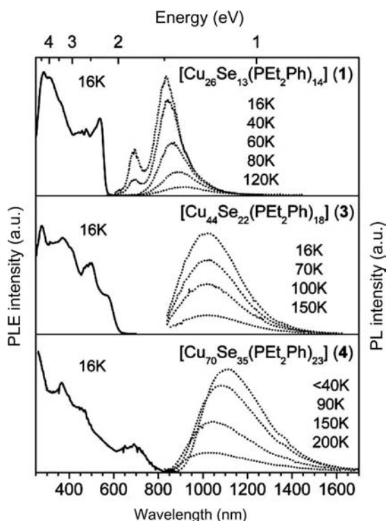
Figure 5.14 Photoluminescence excitation (PLE) spectra (solid lines) and photoluminescence (PL) spectra (dotted lines) of [Cu 26 Se 13 (PEt 2 Ph) 14 ] ( 1 ), [Cu 44 Se 22 (PEt 2 Ph) 18 ] ( 3 ), and [Cu 70 Se 35 (PEt 2 Ph) 23 ] ( 4 ) measured at different temperatures.
