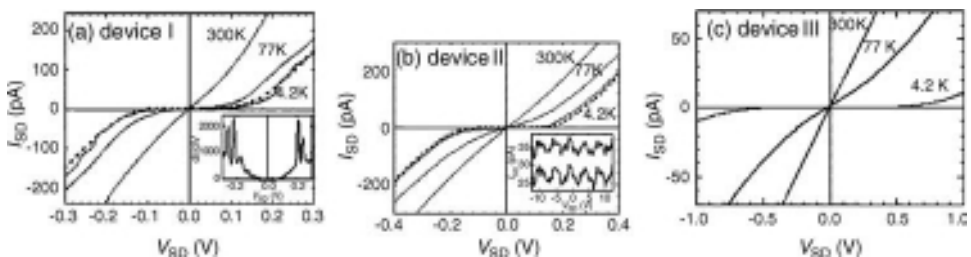
Figure 5.47 I(V) characteristics of devices I–III. (a) 11-mer; (b) 22-mer; (c) 30-mer DNA strands. Reprinted with permission from Ref. [64]; © 2005, American Institute of Physics.
