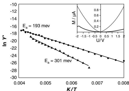
Figure 5.63 Arrhenius plots of samples prepared by specific (triangles) and nonspecific (dots) immobilization. The inset shows the corresponding I(V) curves for specific (gray
