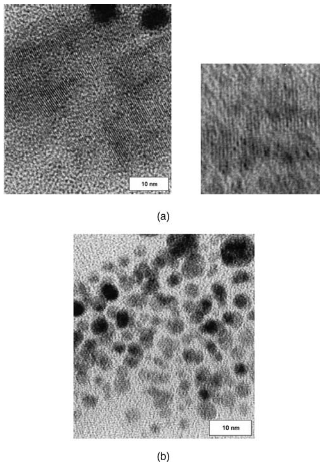
Figure 4.28 (a) TEM image of gold nanowires, consisting of 0.6–0.7 nm particles (see magnified cutout) arranged equidistantly (0.5 nm); (b) The same area after continued electron-beam irradiation, showing the formation of large gold nanoparticles from the wires.
