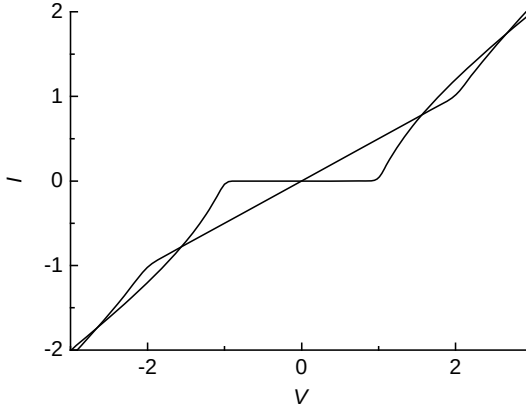
Figure 2.16 Calculated current–voltage ( I – V ) curves for a single-electron transistor for two different values of the gate charge. The source and drain tunnel resistances and capacitances are assumed equal, the charging energy is 100 k_B T . For gate charge Q_G = 0 , the single-electron transistor is in the Coulomb blockade regime, and the I – V curve exhibits the
