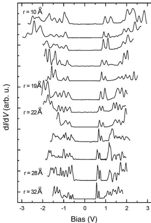
Figure 5.3 Size evolution of the tunneling spectra at 4.2 K of single InAs QDs, displaced vertically for clarity. The position of the centers of the zero-current gap showed nonsystematic variations with respect to the zero bias, of the
