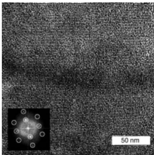
Figure 4.22 TEM image of a cutout of cubically organized \text{Au}_{55}(\text{PPh}_3)_{12}\text{Cl}_6 on PVP. The insert shows the diffraction pattern calculated from the recorded image.
