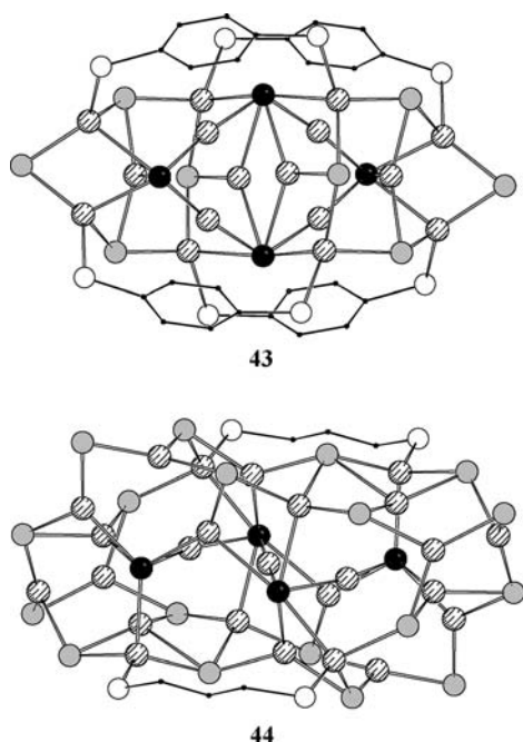
Figure 3.56 Molecular structures of [\text{Cu}_{16}\text{Se}_4(\text{SePh})_8(\text{dppbe})_4] ( 43 ) and [\text{Cu}(\text{dppp})_2][\text{Cu}_{25}\text{Se}_4(\text{SePh})_{18}(\text{dppp})_2] ( 44 ) (without terminal phenyl groups). Cu: shaded spheres; Se: black spheres; SeR: gray spheres; P: white spheres; C: small black spheres.
