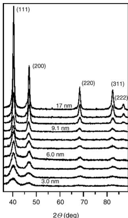
Figure 3.123 Size-dependent evolution of powder XRD patterns for \text{CoPt}_3 nanocrystals. The average nanocrystal sizes were calculated using the Debye–Scherrer equation. Reproduced with permission from Ref. [55]; © 2003, American Chemical Society.
