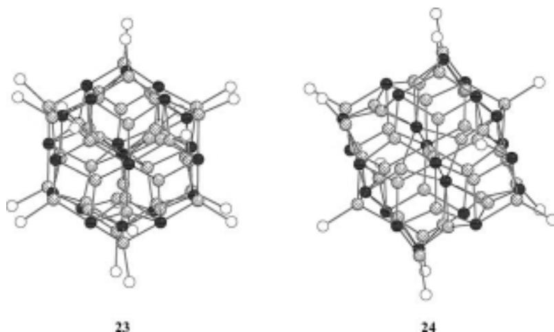
Figure 3.48 Molecular structures of [\text{Cu}_{44}\text{Se}_{22}(\text{PEt}_2\text{Ph})_{18}] ( 23 ) and [\text{Cu}_{44}\text{Se}_{22}(\text{PnButBu}_2)_{12}] ( 24 ) (without organic groups). Cu: shaded spheres; Se: black spheres; P: white spheres.
