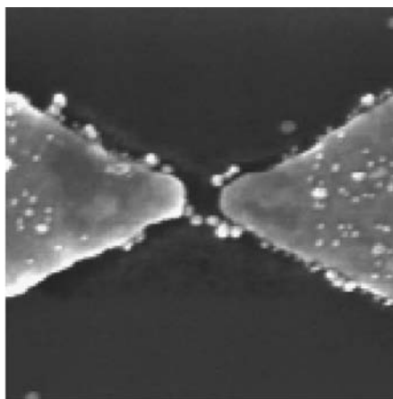
Figure 5.50 Scanning electron microscopy image of a pair of nanoelectrodes with gold nanoparticles immobilized into the gap using a mixture of large and small particles derivatized
