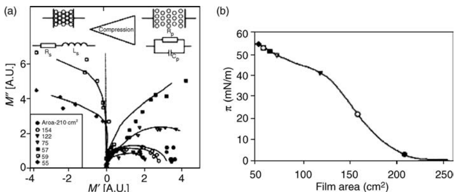
Figure 5.57 (a) Complex impedance response (plot of the imaginary part of the complex modulus M'' versus the real part M' in the complex plane) of a monolayer (3.5 nm diameter) of propanethiol-capped Ag nanoparticles. The particle film response is characterized initially by an RC circuit equivalent, in conformity with a picture of capacitively determined hopping localized conductivity. As the particles are compressed to a separation of less than 0.6 nm, the film becomes inductive, indicating the presence of
