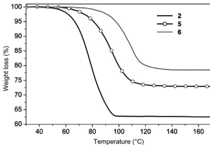
Figure 5.16 Thermogravimetric analysis of [\text{Cu}_{26}\text{Se}_{13}(\text{PET}_3)_{14}] ( 2 ), [\text{Cu}_{70}\text{Se}_{35}(\text{PET}_3)_{23}] ( 5 ) and [\text{Cu}_{140}\text{Se}_{70}(\text{PET}_3)_{34}] ( 6 ) under vacuum conditions.
