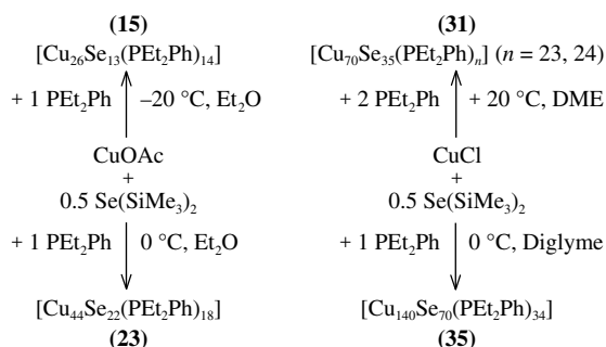
Scheme 3.6 Synthesis of various copper selenide clusters in the presence of \text{PEt}_2\text{Ph} under different reaction conditions.
