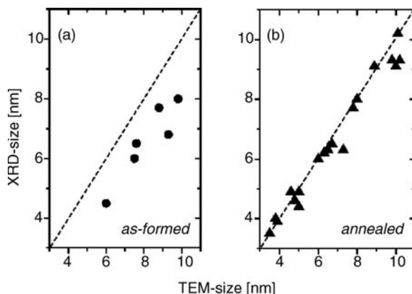
Figure 3.118 In situ annealing of the \text{CoPt}_3 nanoparticles. Comparison of the XRD- and TEM-sizes before and after annealing. Reproduced with permission from Ref. [55]; © 2003, American Chemical Society.
