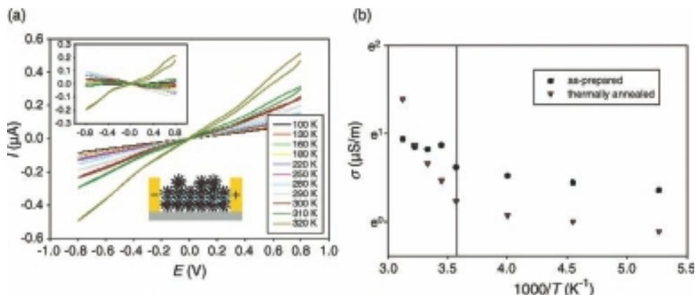
Figure 5.69 (a) I(V) characteristics measured from a Au nanoparticle film at different temperatures after thermal annealing at 340 K for 3 h. The inset shows the difference spectra between as-prepared and annealed films; (b) Film conductivity measured as a function of
