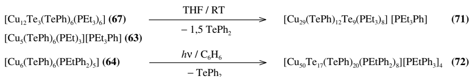
Scheme 3.9 Reaction pathways for the formation of larger telluride–tellurolato-bridged copper clusters, starting from cluster precursors.
