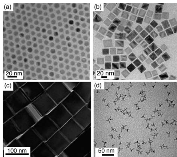
Figure 3.131 TEM images of various shaped iron oxide nanocrystals. (a) 12 nm \text{Fe}_3\text{O}_4 spheres. Reproduced with permission from Ref. [101]; © 2004, Nature Publishing Group; (b) 22 nm \text{Fe}_3\text{O}_4 cubes. Reproduced with permission from Ref. [106]; © 2007, American
