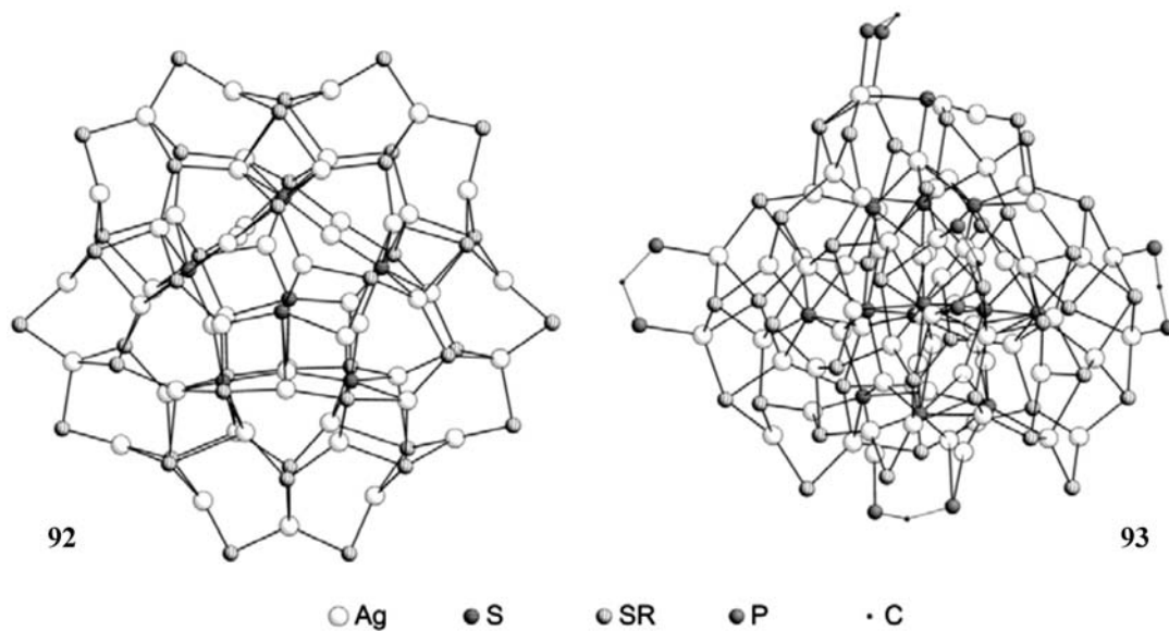
Figure 3.72 Molecular structures of [\text{Ag}_{50}\text{S}_7(\text{SC}_6\text{H}_4\text{tBu})_{40}]^{4-} in 92 (left) and [\text{Ag}_{65}\text{S}_{13}(\text{SC}_6\text{H}_4\text{NMe}_2)_{28}(\text{dppm})_5] 93 (right), without organic groups at the RS ligands.
