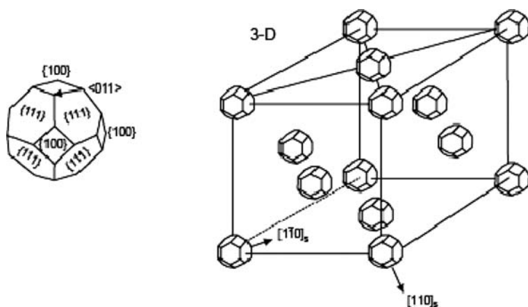
Figure 4.7 Sketch of a superlattice of truncated octahedral 5.0 nm Ag nanoparticles.
