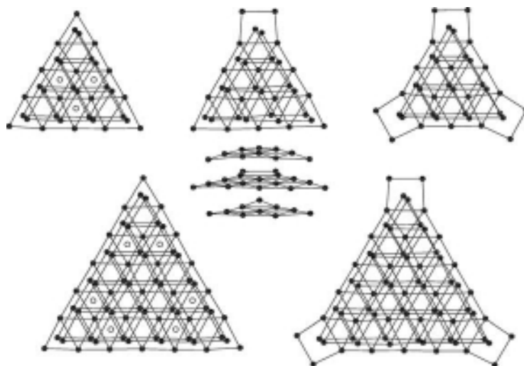
Figure 3.50 Selenium substructures in 28 , 32 , 33 , 34 , and 36 (from top left to bottom right) which contain 35, 36, 38, 70, or 73 selenium atoms. The drawn Se–Se contacts do not represent binding interactions, but only serve to visualize the A–B–A packing of
