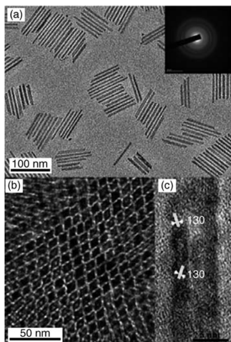
Figure 3.132 (a) TEM image of goethite ( \alpha\text{-FeOOH} ) nanotubes; (b) Superlattice of ordered goethite nanotubes; (c) HR-TEM image of goethite nanotubes. Reproduced with permission from Ref. [123]; © 2007, American Chemical Society.
