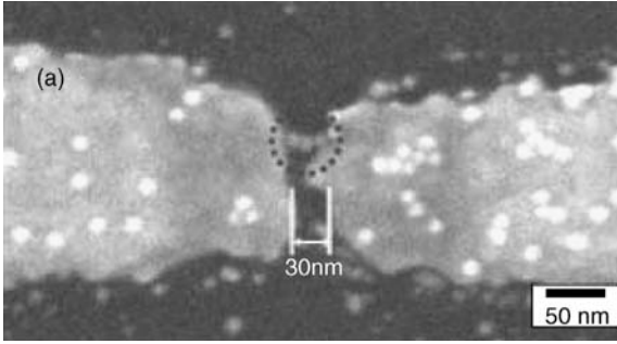
Figure 5.46 Field-emission SEM image of a fabricated device. Reprinted with permission from Ref. [64]; © 2005, American Institute of Physics.
