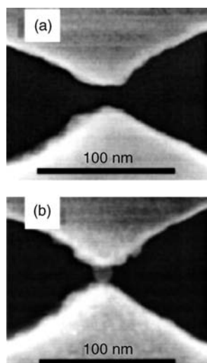
Figure 5.36 (a) Pt electrodes (white) separated by a \sim 14 nm gap; (b) After electrostatic trapping, the same electrodes are bridged by a single \sim 17 nm Pd particle. Reprinted with permission from Ref. [51]; © 1997, American Institute of Physics.
