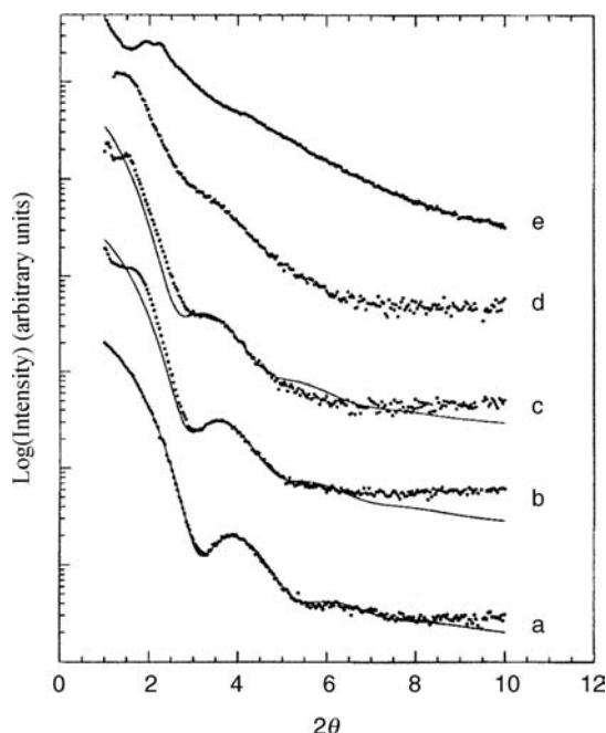
Figure 3.16 Small-angle X-ray scattering data from bare 4.2 nm CdSe particles (a) overgrown by 0.65 (b) through 5.3 (e) monolayers of ZnS. From Ref. [274].
