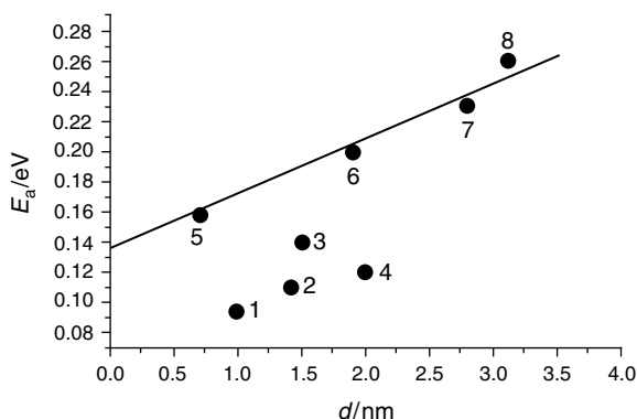
Figure 5.68 Diagram of activation energy measured in dependence of the cluster–cluster distance. Reproduced with permission from Ref. [107]; © 2003, Wiley-VCH Verlag GmbH & Co. KGaA.
