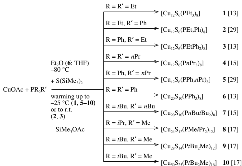
Scheme 3.3 Survey of the synthesis of sulfur-bridged copper clusters protected by terminal phosphine ligands.
