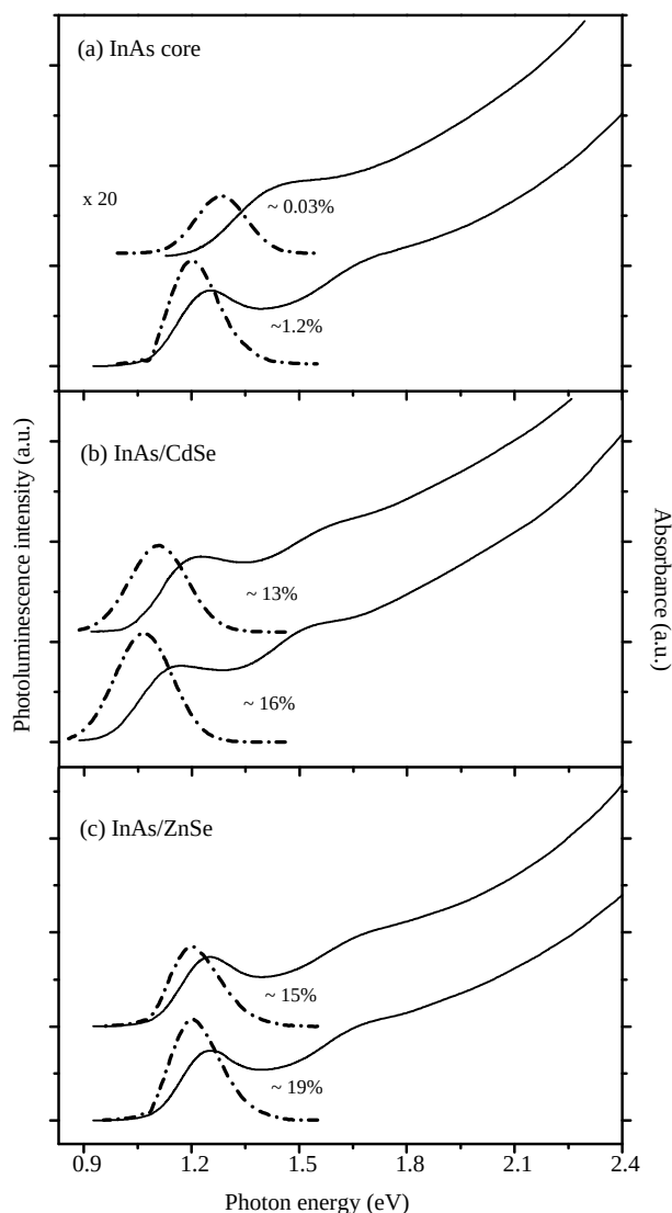
Figure 3.35 Comparison of stability of (a) cores, (b) InAs–CdSe core–shells, and (c) InAs–ZnSe core–shells. The absorption spectra (solid lines) and PL spectra (dashed lines) are shown on the same energy scale for fresh
