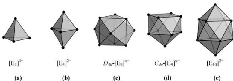
Figure 3.1 Structures of known homoatomic tetrel clusters.
