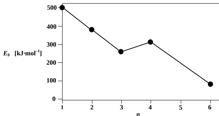
Figure 3.41 Course of the Cu–P binding energies per Cu–P bond E_b in phosphine-ligated clusters [\text{Cu}_{2n}\text{S}_n(\text{PH}_3)_m] ( n = 1-4, 6 ; m = 2, 4, 6, 8 ). The given values consider the
