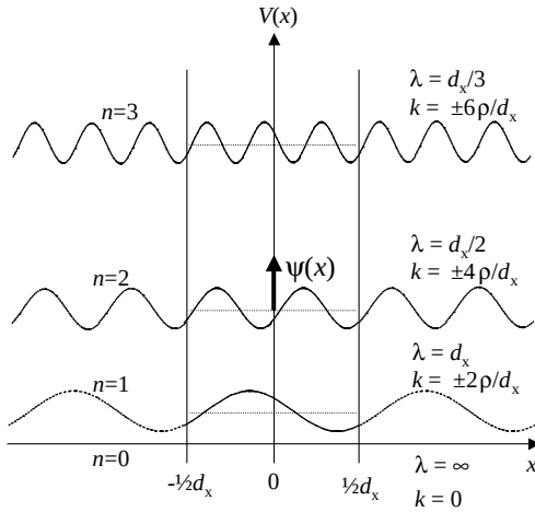
Figure 2.2 Periodic boundary conditions (drawn only for the x -dimension) for a free electron gas in a solid with thickness d . The idea of periodic boundary conditions is to mathematically “simulate” an infinite solid. Infinite extension is similar to an object without any borders; this means that a particle close to the “border” must not be affected by the border, but “behaves” exactly as in the bulk. This can be realized by using a wavefunction \psi(x) that is periodic within the thickness d of the solid. Any electron that leaves the solid from its right
