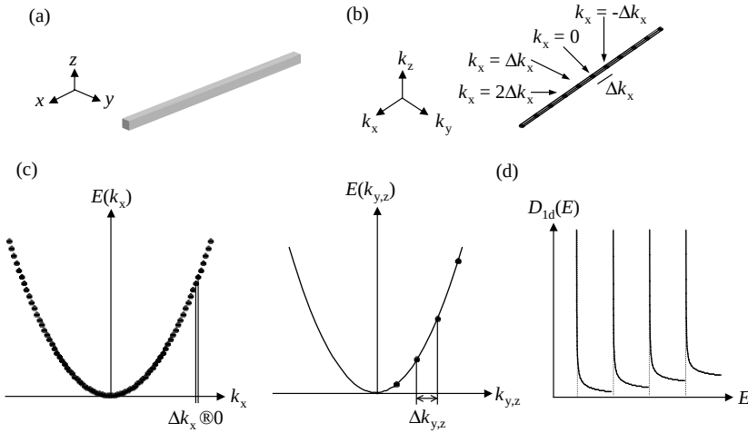
Figure 2.6 (a) A one-dimensional solid; (b) The allowed (k_x, k_y, k_z) -states can be visualized as lines parallel to the k_x -axes in the 3-D k -space. In this figure, only one line is shown as an example. Within each line, the distribution of states is quasi-continuous, since \Delta k_x \rightarrow 0 . The arrangement of the individual lines is discrete, since only certain discrete k_y - and k_z -
