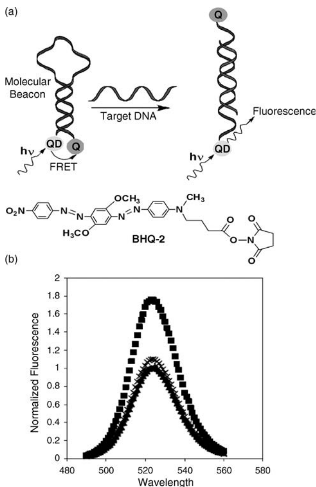
Figure 6.17 (a) Optical detection of DNA by a hairpin nucleic acid functionalized with QDs and quencher units Q; (b) Fluorescence intensities: \blacklozenge without target DNA, \blacksquare with target DNA, \blacktriangle single-base mismatched target DNA (SMT), \times noncomplementary target DNA (NST). (Reproduced with permission from IOP Publisher from ref. [159]).
