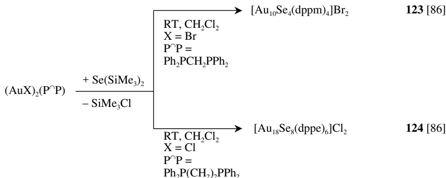
Scheme 3.19 The synthesis of selenido-bridged gold clusters with bidentate phosphine ligands.
