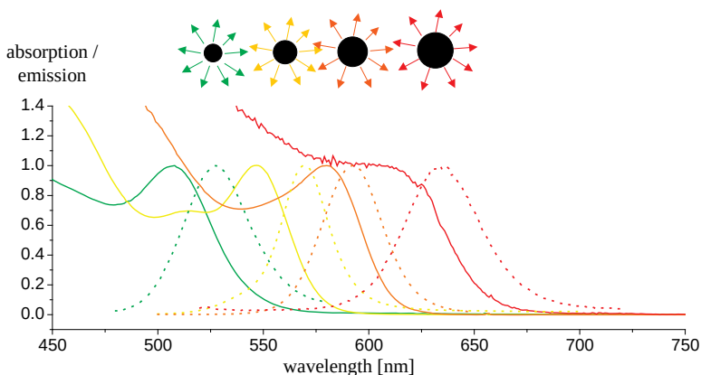
Figure 2.11 Absorption (solid lines) and emission spectra (dotted lines) of colloidal CdSe QDs of different sizes. The absorption peak of green/yellow/orange/red
