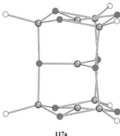
Figure 3.96 The Ag–Te–P framework in [\text{Ag}_9(\text{TePh})_9(\text{PEt}_2\text{Ph})_6] ( 117a ) (without organic groups). Ag: shaded spheres; TeR: gray spheres; P: white spheres.
