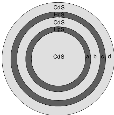
Figure 3.19 Schematic drawing of the double-well nanoheterostructures described in the text. The wells (a and c) consist of the small bandgap material \beta -HgS, the core, the barrier between the wells (b) and the cladding layer (d) are made from CdS. From Ref. [208].
