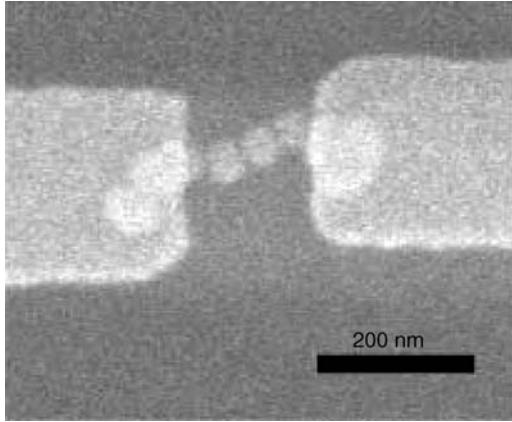
Figure 5.48 Two-island device fabricated by contacting a self-assembled chain of nanoparticles. The two particles framing the two island particles form part of the electrodes, such
