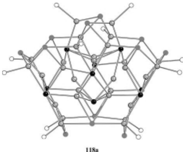
Figure 3.97 A projection of the core atoms in [\text{Ag}_{30}(\text{TePh})_{12}\text{Te}_9(\text{PEt}_3)_{12}] ( 118a ). Ag: shaded spheres; Te: black spheres; TeR: gray spheres; P: white spheres.
