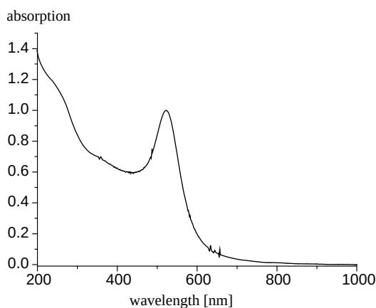
Figure 2.13 Absorption spectrum of colloidal gold nanocrystals of 10 nm diameter.
