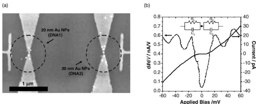
Figure 5.38 (a) SEM image of single 20 and 30 nm-diameter Au nanoparticles assembled from solution and bridging the two adjacent nanoelectrode junctions; (b) Current–voltage ( I(V) ) characteristics and corresponding conductance (numerical dI/dV ) plot for a DPN-generated nanopag device assembled
