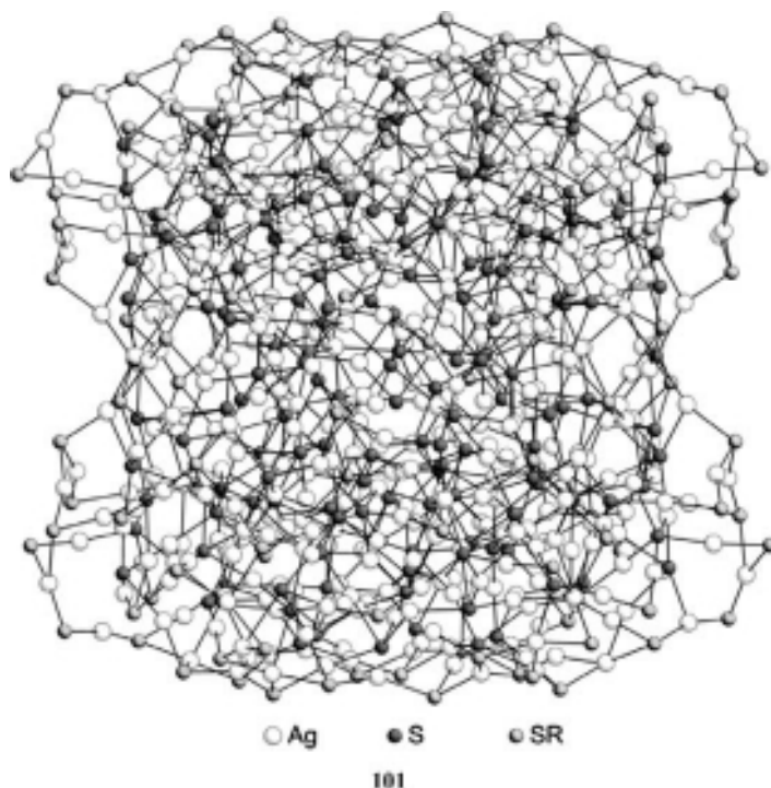
Figure 3.76 The molecular structure of [\text{Ag}_{490}\text{S}_{188}(\text{StC}_5\text{H}_{11})_{114}] ( 101 ) without organic groups.
