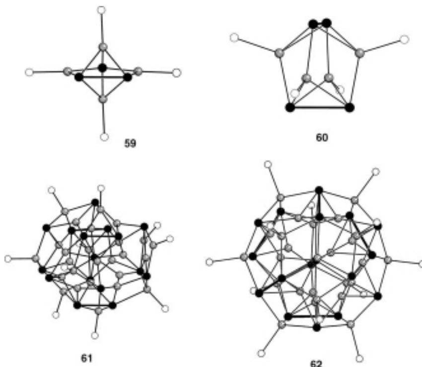
Figure 3.67 Molecular structures of stoichiometric copper telluride clusters [\text{Cu}_4\text{Te}(\text{Te}_2)_2(\text{PCyPh}_2)_4] ( 59 ), [\text{Cu}_4(\text{Te}_2)_2(\text{P}i\text{Pr}_3)_4] ( 60 ), [\text{Cu}_{26}\text{Te}_{10}(\text{Te}_2)_3(\text{PtBu}_3)_{10}] ( 61 ), and
