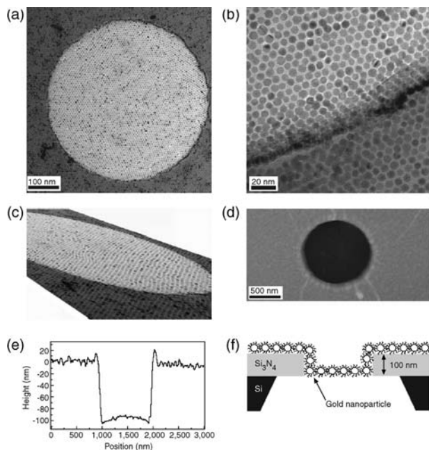
Figure 5.59 (a) TEM image of a free-standing array with a diameter of 250 nm; (b) A higher-magnification image of the membrane; (c) TEM image of a tilted membrane; (d) AFM height image of a free-standing membrane with a
