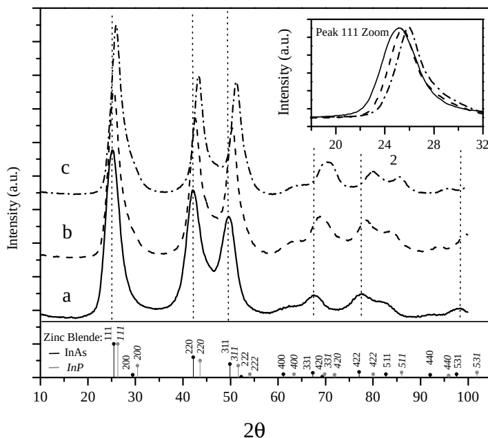
Figure 3.32 X-ray diffraction patterns for InAs cores with radius of 1.7 nm (trace a, solid line), and InAs-InP core-shells with shell thickness of 2.4 monolayers (trace b, dashed line), and 6.2 monolayers (trace c, dot-dashed line). The inset
