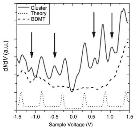
Figure 5.26 Conductance curves dI/dV(V) taken on an individual cluster deposited on a self-assembled monolayer of 1,4-benzenedimethanethiol (BDMT) on Au(111). Both, equidistant Coulomb charging peaks and nonequidistant peaks (indicated by the arrows) are observed. The latter peaks are attributed to discrete electronic levels caused by the electron
