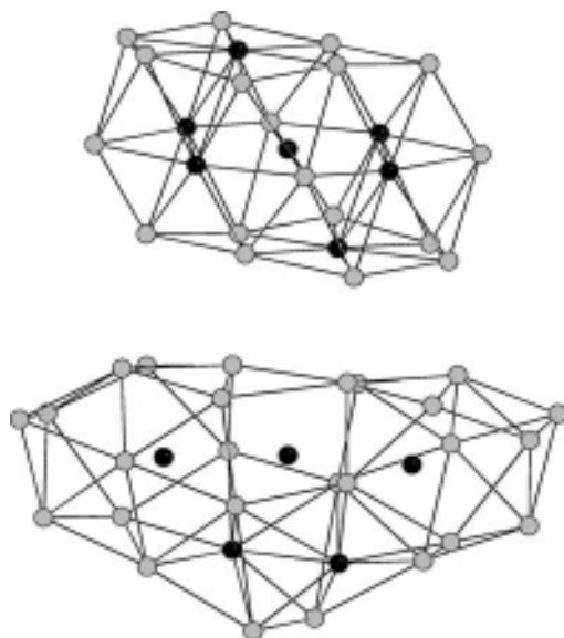
Figure 3.58 Selenium substructures in 45 (top) and 46 (bottom). Se: black spheres; SeR: gray spheres. The drawn Se–Se contacts do not represent bonding interactions, but only serve
