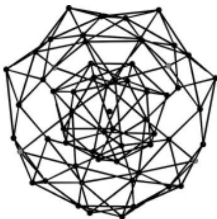
Figure 3.87 The selenium substructure in 108 . The central Se atom is surrounded by the \text{Se}_{16} Frank–Kasper polyhedron, which is itself surrounded by the \text{Se}_{44} polyhedron in a second coordination sphere.
