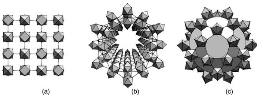
Figure 3.10 Proposed Ge allotropes based on \text{Ge}_9 building units. (a) Two-dimensional connection of nido - \text{Ge}_9 clusters forming a \{^2_\infty[\text{Ge}_9]_n\} sheet; [88] (b) \{^1_\infty[\text{Ge}_9]_n\} nanotube composed of \text{Ge}_9 clusters. The unit cell of the tube is composed of six unit cells of the sheet shown in Figure 3.10a; (c) (\text{Ge}_9)_{30} cage derived from a truncated icosadodecahedron [87].
