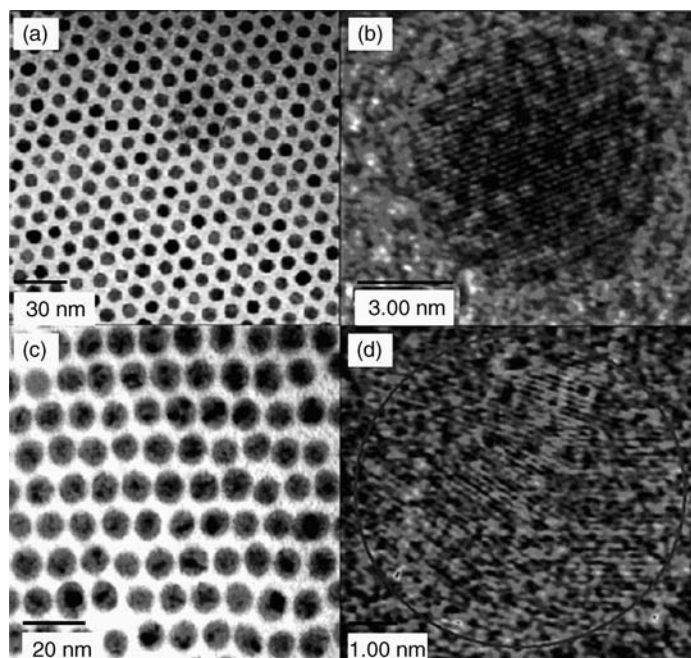
Figure 3.116 TEM images of cobalt nanoparticles. (a) Low-magnification image of \epsilon -Co. The even contrast across the individual particles implies a uniform crystalline structure for this phase; (b) HR-TEM image of \epsilon -Co, showing perfect crystallographic coherence and discrete faceting; (c) Low-magnification image
