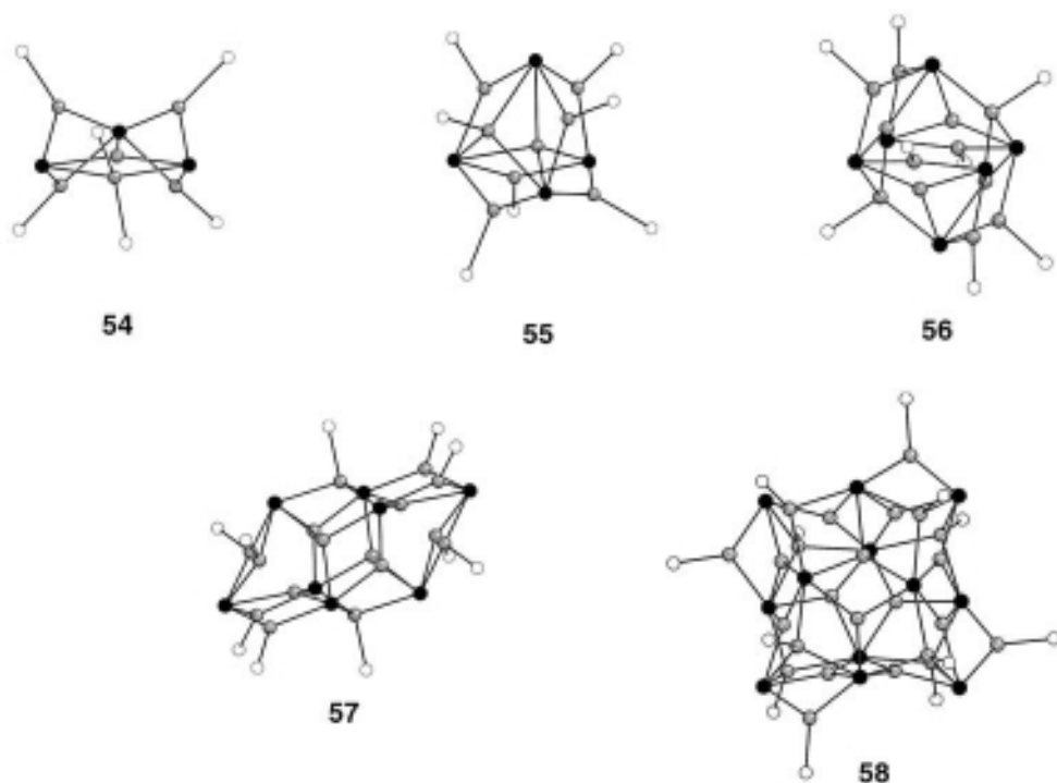
Figure 3.66 Molecular structures of stoichiometric copper telluride clusters [\text{Cu}_6\text{Te}_3(\text{PCyPh}_2)_5] ( 54 ), [\text{Cu}_8\text{Te}_4(\text{PPh}_3)_7] ( 55 ), [\text{Cu}_{12}\text{Te}_6(\text{PPh}_3)_8] ( 56 ), [\text{Cu}_{16}\text{Te}_8(\text{PPhnPr}_2)_{10}]
