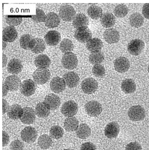
Figure 3.119 HR-TEM image of annealed \text{CoPt}_3 nanocrystals. Note that almost all nanoparticles possess the lattice fringes without stacking faults and other defects.
