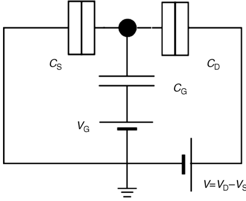
Figure 2.14 A schematic circuit diagram for a single-electron transistor. The electron island, indicated by the black dot, is connected to source and drain contacts via tunneling barriers having capacitances C_S and C_D . Additionally, the
