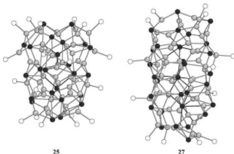
Figure 3.49 Molecular structures of [\text{Cu}_{48}\text{Se}_{24}(\text{PMe}_2\text{Ph})_{20}] ( 25 ) and [\text{Cu}_{59}\text{Se}_{30}(\text{PCy}_3)_{15}] ( 27 ) (without organic groups). Cu: shaded spheres; Se: black spheres; P: white spheres.
