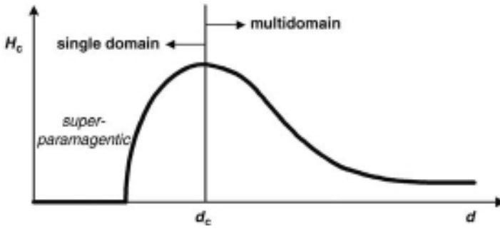
Figure 3.143 Particle coercivity versus size. The largest coercivity is observed at the particle size d_c , corresponding to the transition from multidomain to single-domain structure.
