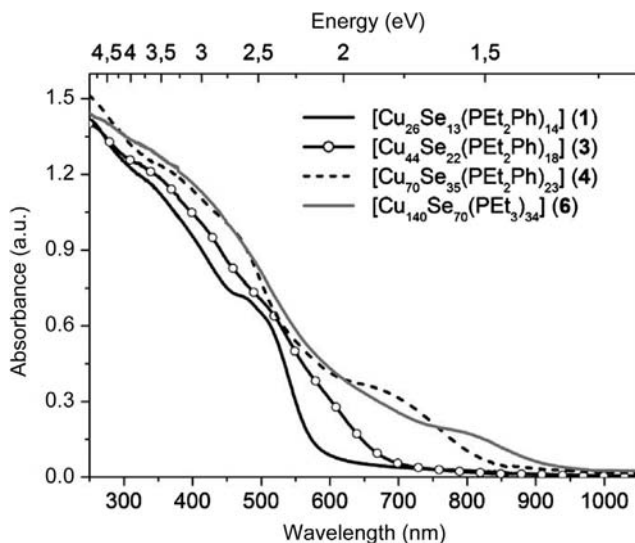
Figure 5.13 Solid state absorption spectra of \text{PET}_2\text{Ph} - or \text{PET}_3 -ligated compounds 1 , 3 , 4 , and 6 . For the measurements, single crystalline samples, previously pulverized in mineral oil, were placed between two quartz plates.
