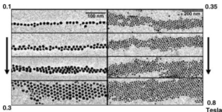
Figure 4.40 TEM images of 1-D ordered cobalt nanoparticles self-assembled in the magnetic fields of different strengths. Reproduced with permission from Ref. [30]; © 2002, Elsevier Science.
