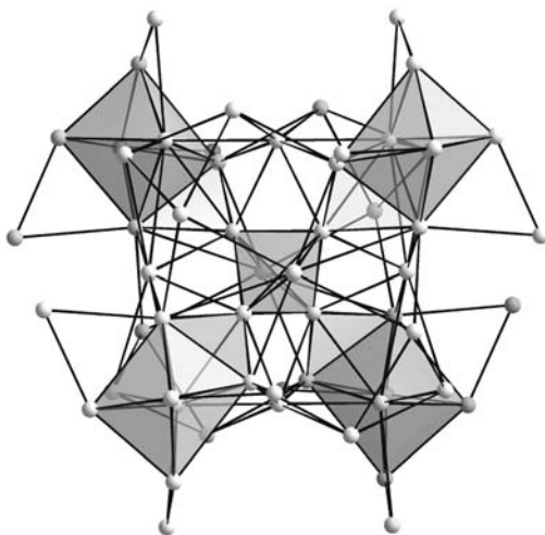
Figure 3.63 Copper substructure in 52 . The connected tetrahedra \text{Cu}_4 and octahedra \text{Cu}_6 are highlighted by gray shading. Cu–Cu distances are drawn up to 3.012 Å.
