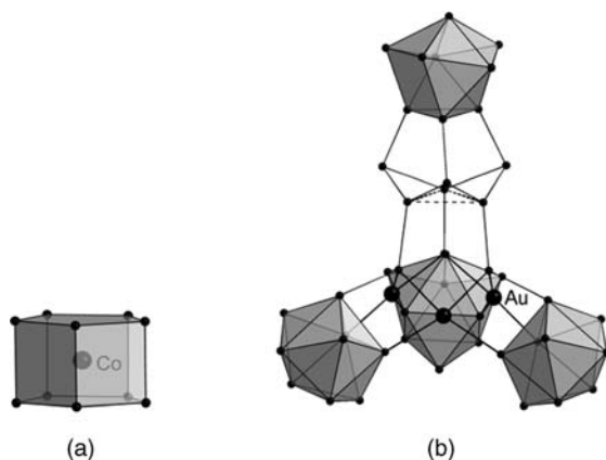
Figure 3.9 (a) The nondeltahedral endohedrally filled anion [\text{Co}@\text{Ge}_{10}]^{3-} [81]; (b) The largest structurally characterized cluster of heavier tetrel elements [\text{Au}_3\text{Ge}_{45}]^{9-} [86].
