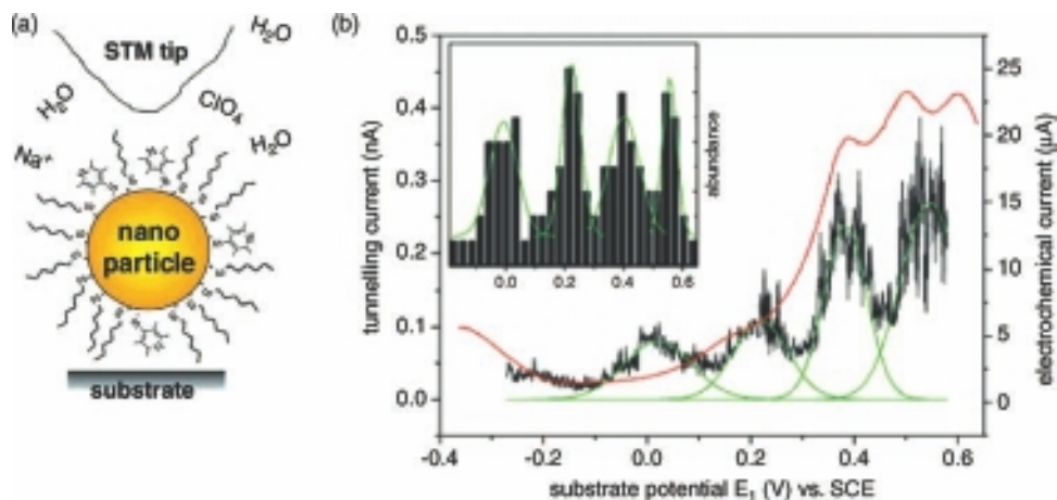
Figure 5.33 (a) Monolayer-protected nanoparticle in an electrochemical in situ STM configuration; (b) Sequential charging events observed in DPV (red) and I_t(\eta) tunneling spectroscopy (black) at constant V_{\text{bias}} = 0.05 V ( I_{\text{set}}^0 = 0.05 nA). Inset: Abundance distribution
