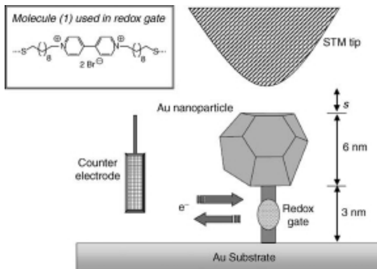
Figure 5.31 Scheme describing the redox switch, which is based on a viologen redox center incorporated within the nanoparticles ligand shell. Reprinted with permission from Ref. [46]; © 2000, Macmillan Publishers Ltd.
