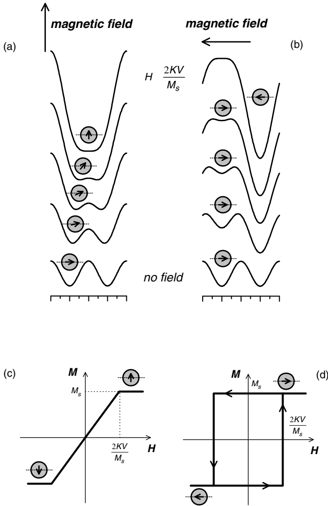
Figure 3.141 (a,b) Dependence of potential energy on the direction of a particle magnetic moment in presence of external magnetic fields applied (a) perpendicular and (b) parallel to the easy magnetization axis. The lower curves correspond to zero magnetic field, and the upper curves to the saturation magnetization
