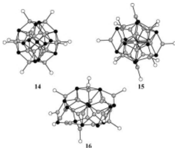
Figure 3.42 Molecular structures of [\text{Cu}_{20}\text{Se}_{13}(\text{PEt}_3)_{12}] ( 14 ), [\text{Cu}_{26}\text{Se}_{13}(\text{PEt}_2\text{Ph})_{14}] ( 15 ), and [\text{Cu}_{26}\text{Se}_{13}(\text{PCy}_3)_{10}] ( 16 ) (without organic groups). Cu: shaded spheres; Se: black spheres; P: white spheres.
