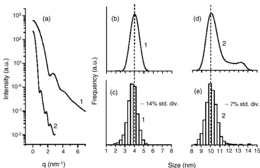
Figure 3.122 (a) The angular dependence of scattered X-ray intensity (SAXS) from two samples of as-prepared \text{CoPt}_3 nanocrystals with mean size (1) \sim 4 nm and (2) \sim 10 nm; (b and d) Particle volume fraction versus size curves
