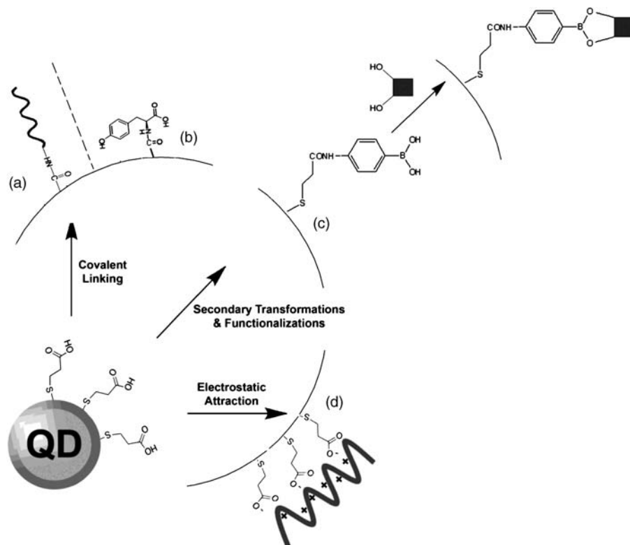
Figure 6.3 Modification of monolayer-functionalized QDs with molecular or macromolecular components. (a, b) Covalent attachment; (c) Attachment of ligand; (d) Electrostatic association of a polymer.
