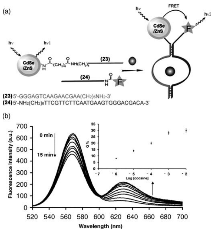
Figure 6.21 (a) QD-based optical sensing of cocaine by the formation of a cocaine–aptamer subunit supramolecular structure that stimulates a FRET process; (b) Time-dependent luminescence spectra of the system consisting of the 23 -functionalized QDs and Atto 590-modified 24 , upon interaction with cocaine,
