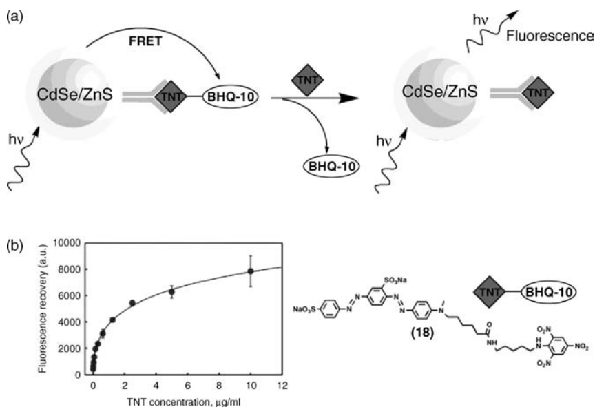
Figure 6.15 (a) Competitive analysis of TNT by the anti-TNT antibody associated with CdSe/ZnS QDs and using BHQ-10 as quencher; (b) Derived calibration curve for the analysis of TNT. (Reproduced with permission from ref. [153]. Copyright 2005 American Chemical Society).
