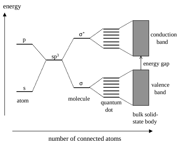
Figure 2.1 Electronic energy levels depending on the number of bound atoms. By binding more and more atoms together, the discrete energy levels of the atomic orbitals merge into energy bands (here
