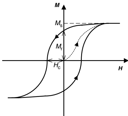
Figure 3.139 A typical hysteresis loop for a ferromagnetic material and the important magnetic parameters which can be obtained from the hysteresis loop. The dotted line shows the first scan.
