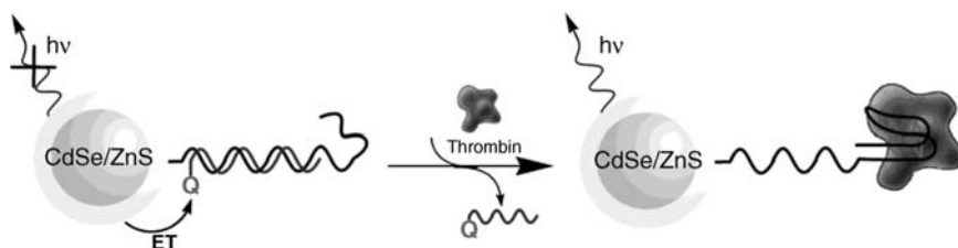
Figure 6.19 Optical analysis of thrombin by the formation of the aptamer–thrombin complex, and separation of the quencher-nucleic acid blocking unit.
