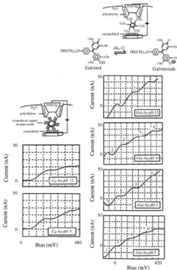
Figure 5.32 Current–voltage curves for C 8 -Au (left) and Gal-Au (right) in H 2 O as a function of pH (adjusted with phosphate buffer, see Ref. [6]). The numbers 1–4 in the Gal-Au data identify voltage plateaus. Cartoons of the experimental arrangements for measuring I – V curves of individual nanoparticles in solution
