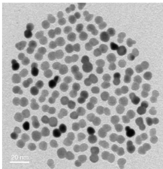
Figure 3.135 TEM image of symmetric Au-CoPt 3 nanocrystals synthesized by a modified procedure as described in Ref. [142].
