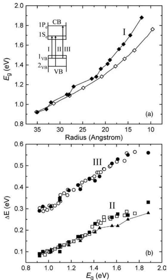
Figure 5.4 Correlation of optical and tunneling spectroscopy data for InAs QDs. The inset shows a schematic of the CB and VB level structure and optical transitions I, II, and III (a,b and c in Figure 5.3). (a) Comparison of the size dependence of the low-temperature optical band gap (transition I) after Coulomb correction (open diamonds), with the band-gap measured by the STM (filled diamonds); (b) Excited transitions plotted versus the band gap for tunneling and optical spectroscopy. The two lower data sets (II) depict the correlation
