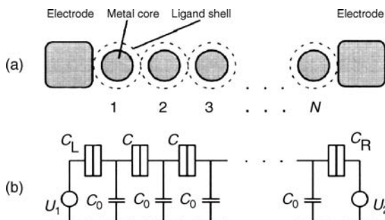
Figure 5.39 (a) 1-D array of N ligand-stabilized metal clusters; (b) The corresponding circuit equivalent. Reprinted with permission from Ref. [53]; © 1997, Elsevier.
