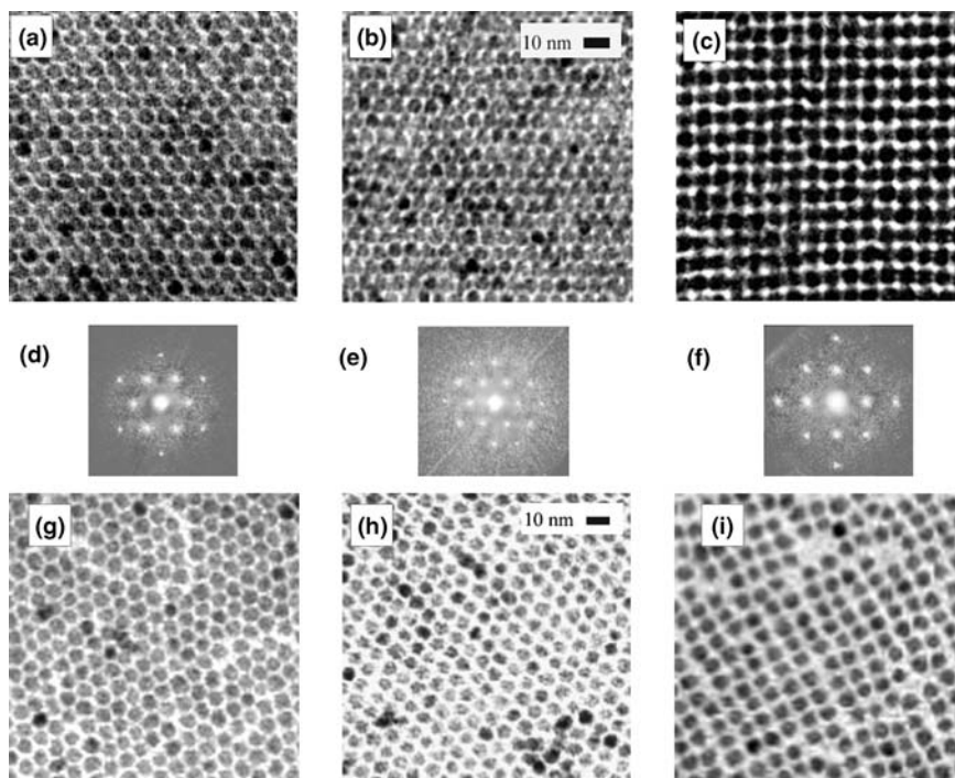
Figure 3.24 TEM images of arrays and superlattices prepared from InAs nanocrystals, 5.8 nm in diameter. Frames (a–c) show ordered superlattices prepared from InAs nanocrystals,
