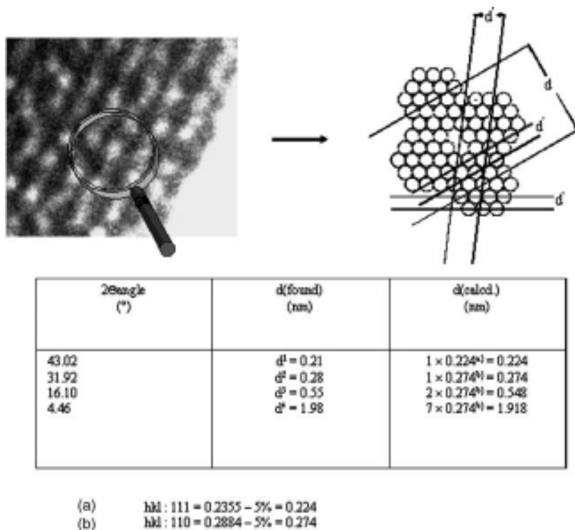
Figure 4.10 Magnified TEM image of an Au 55 microcrystal and crystallographic data from SAXRD and WAXRD studies. The hkl values 111 and 110 are reduced by 5% due to the size-determined contraction of Au–Au distances in small particles.
