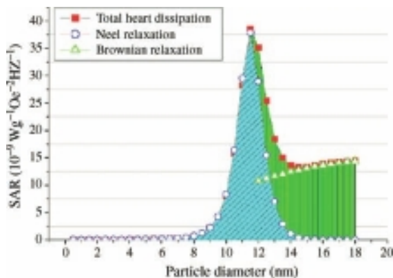
Figure 3.152 Theoretical estimation of the heating rates as a function of particle diameter. The calculations used surfactant layer thickness of 3.2 nm, the anisotropy constant 30 \text{ kJ m}^{-3} , temperature 300 K, viscosity
