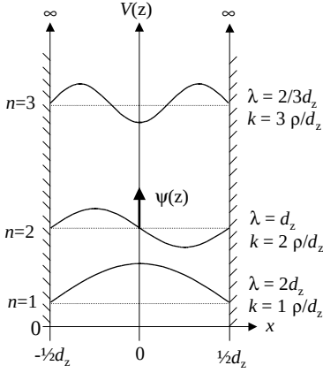
Figure 2.4 Particle in a box model for a free electron moving along in the z axis. The movement of electrons in z -direction is limited to a “box” with thickness d . Since electrons cannot “leave” the solid (the box), their potential energy V(x) is zero within the
