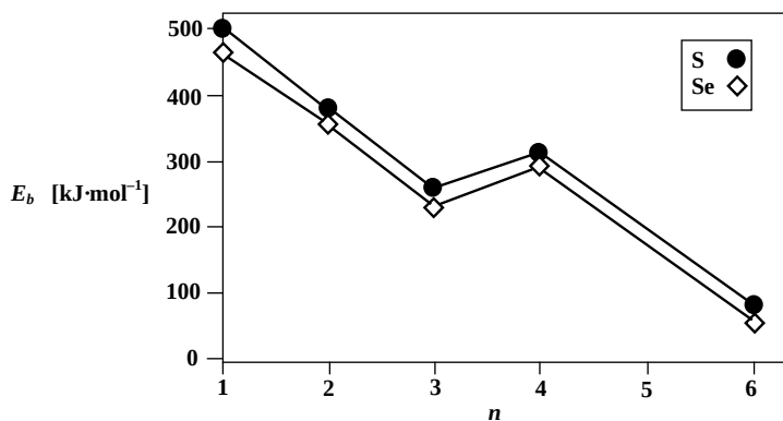
Figure 3.54 Course of the Cu–P binding energies per Cu–P bond E_b in phosphine-ligated clusters [\text{Cu}_{2n}\text{E}_n(\text{PH}_3)_m] ( \text{E} = \text{S}, \text{Se} ; n = 1-4, 6 ; m = 2, 4, 6, 8 ). The given values
