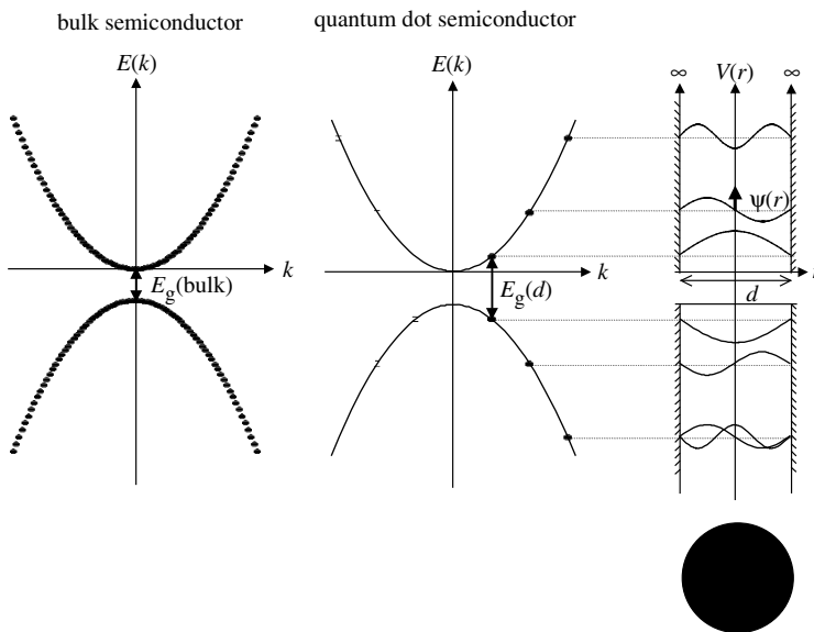
Figure 2.8 Free charge carriers in a solid have a parabolic dispersion relation ( E(k) \propto k^2 ). In a semiconductor, the energy bands for free electrons and holes are separated by an energy gap E_g . In a bulk semiconductor, the states are quasi-continuous, and each point in the energy bands represents an individual state. In a quantum dot (QD), the charges are confined to a small volume. This situation can be described
