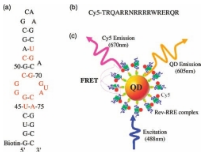
Figure 6.37 (a) Aptamer structure for the Rev regulatory protein; (b) Sequence of the Cy5-labeled Rev peptide; (c) Hybrid consisting of the aptamer-functionalized QDs for the FRET analysis of the Rev peptide. (Reprinted with permission from Ref. [203]. Copyright 2006 American Chemical Society).
