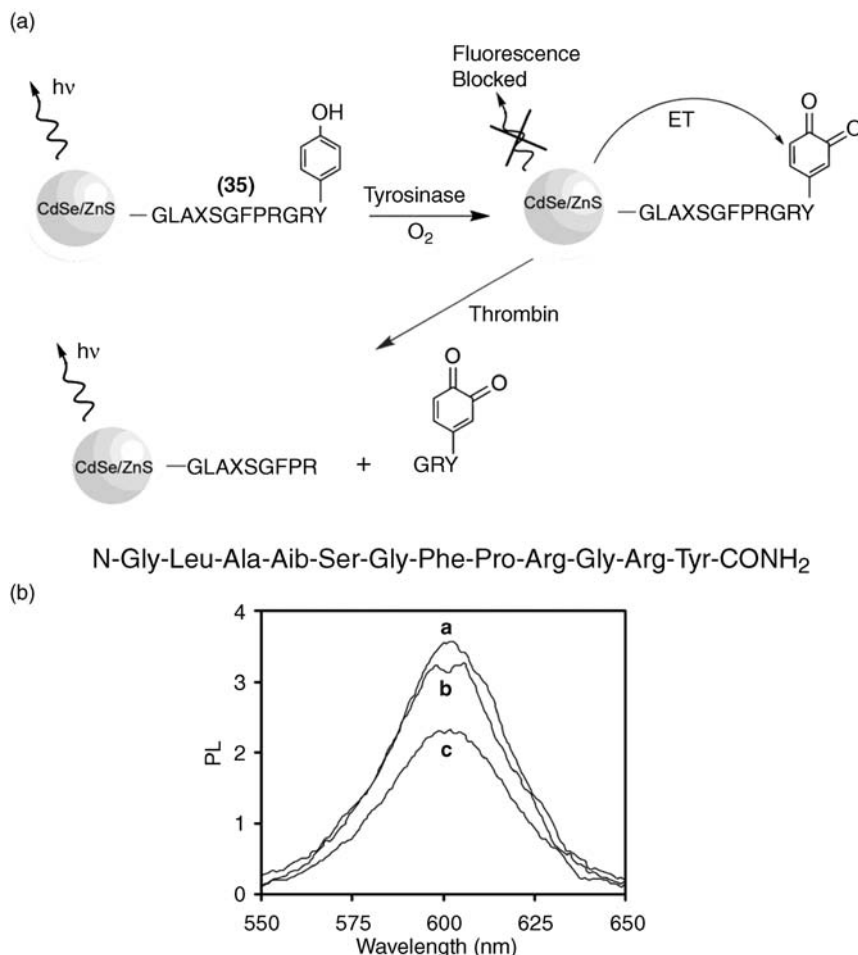
Figure 6.29 (a) Sequential analysis of tyrosinase activity and thrombin activity by the tyrosinase-induced oxidation of the tyrosine-containing peptide 35 associated with the CdSe/ZnS QDs results in electron transfer quenching of the QDs, followed by the thrombin-induced cleavage of the dopaquinone-modified peptide to restore the QDs fluorescence; (b) (spectrum
