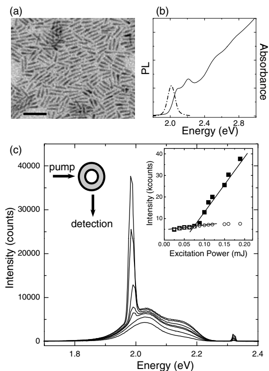
Figure 5.11 (a) A TEM image of the quantum rod sample (scale bar = 50 nm); (b) The absorption (solid line) and emission (dot-dashed line) for the quantum rods (QRs) in solution; (c) Emission spectra for the QRs loaded in the microcavity at different pump powers. The peak at 2.33 eV is the residual scattering of the pump laser. The pump intensities from low to high were: 0.016, 0.038, 0.075, 0.088, 0.10, 0.15, 0.19 mJ. The narrow peak at 1.98 eV emerging above the fluorescence is the laser signal that appears at
