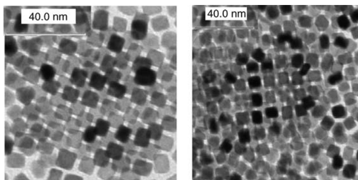
Figure 4.20 TEM images of self-assembled structures of cubic CoPt 3 nanocrystals.
