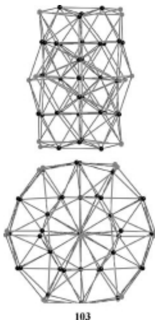
Figure 3.80 Two projections of the \text{Se}_{52} selenium substructure in 103 . Se: black spheres, SeR: gray spheres.
