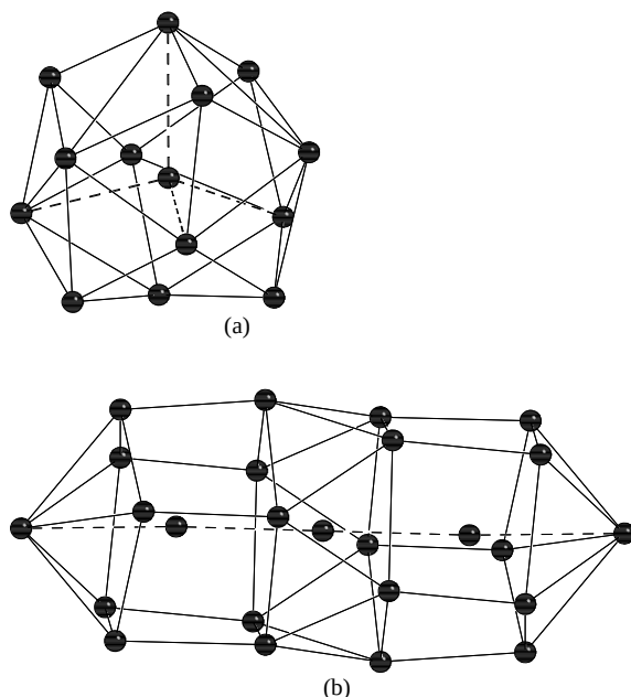
Figure 3.39 S_{14} (a) and S_{25} (b) polyhedra in 9 and 10 , respectively. The drawn S–S contacts do not represent binding interactions, but serve only to explain the geometries of the polyhedra.
