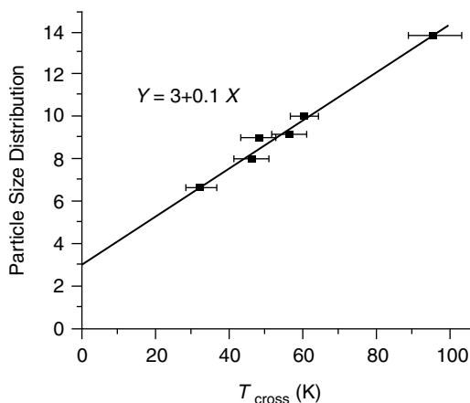
Figure 5.64 Plot of particle size distribution versus transition temperature (crossover point between activated transport mechanism and variable range hopping). Reproduced with kind permission from Ref. [93]; © 2002, American Chemical Society.
