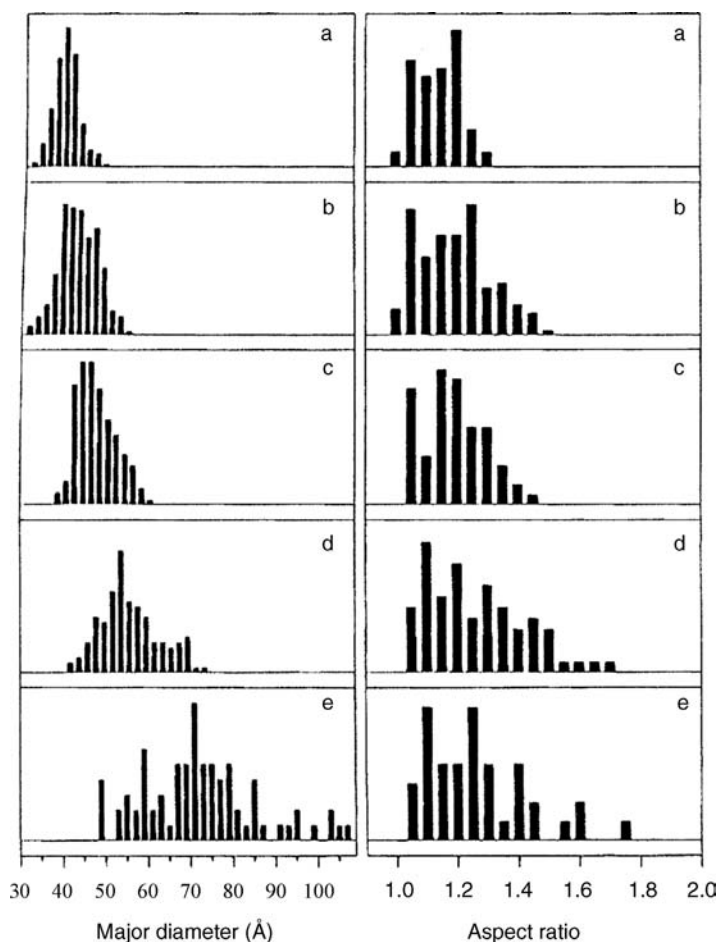
Figure 3.17 Left column: Size histograms of a series of CdSe nanocrystals overgrown with 0.65 (b) to 5.3 (e) monolayers of ZnS (a) and corresponding aspect ratios (right column). From Ref. [274].
