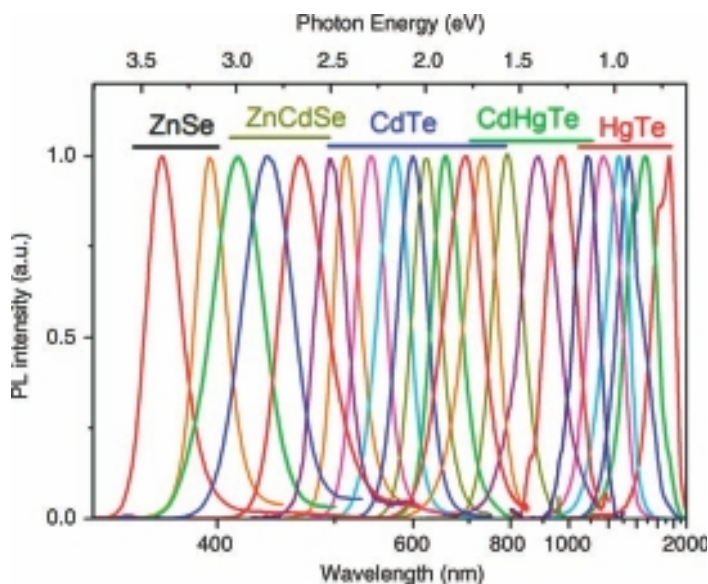
Figure 3.13 Normalized emission spectra of various thiol-capped nanocrystals.
