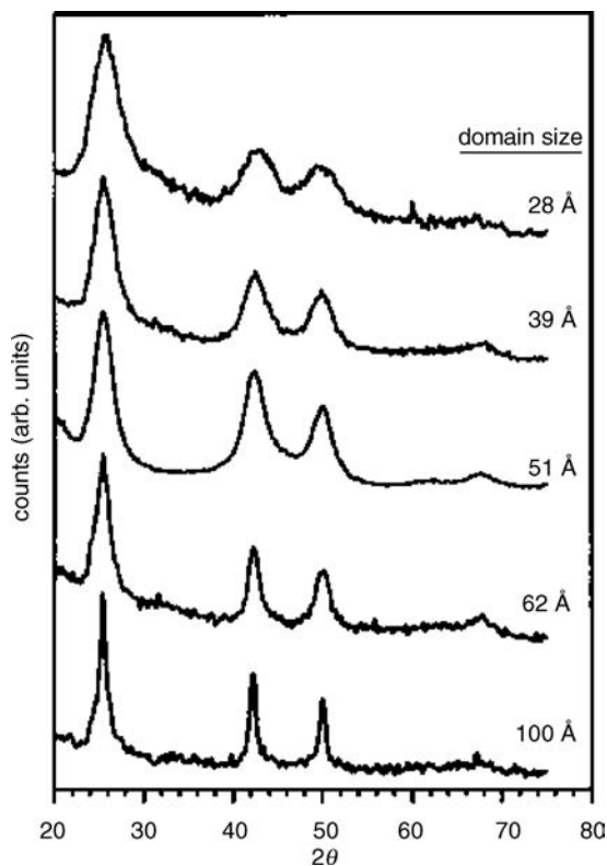
Figure 3.22 Powder X-ray diffraction spectra of InAs nanocrystals with different sizes. The domain size was calculated from the width of the reflections, as detailed in the text. Reproduced from Ref. [188].
