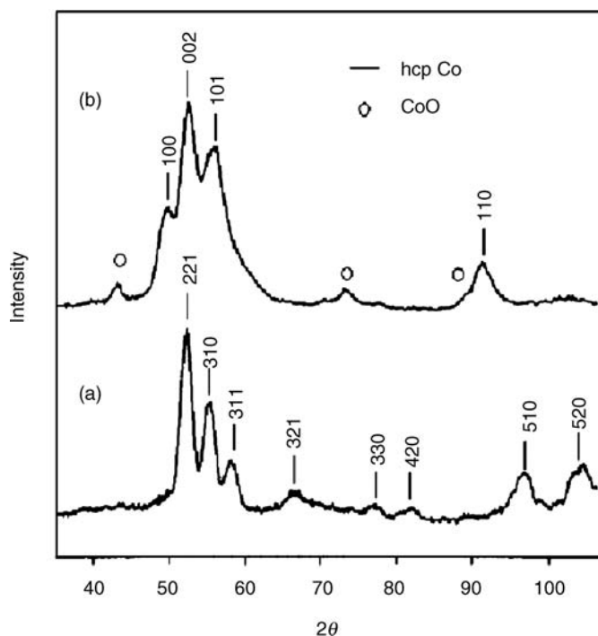
Figure 3.117 XRD patterns of the \epsilon -Co particles before and after annealing. (a) As-synthesized 9 nm particles; (b) After annealing at 300°C under vacuum for 3 h. Reproduced with permission from Ref. [9]; © 1999, American Institute of Physics.
