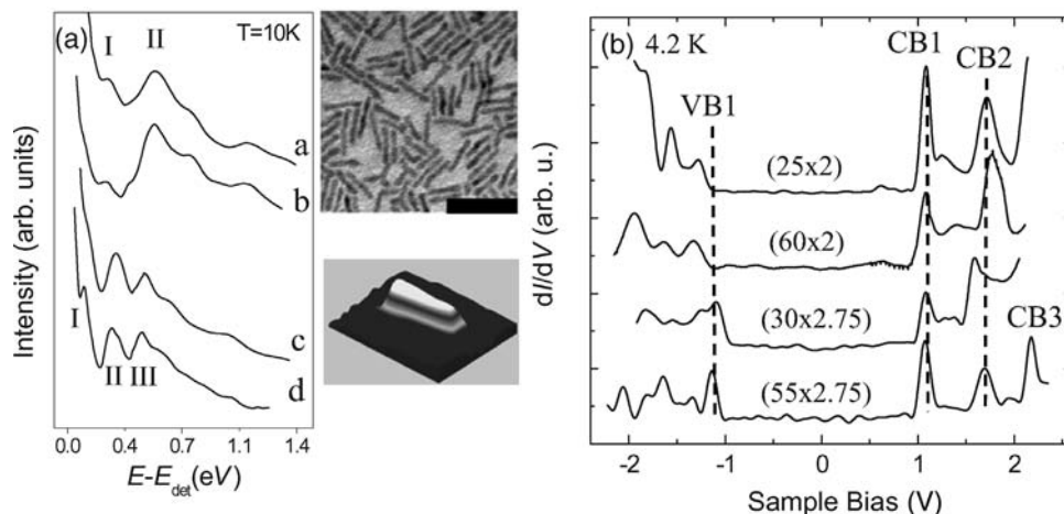
Figure 5.9 (a) Optical and tunneling spectroscopy of CdSe QRs. PLE spectra for CdSe QRs: spectrum (a) 31 \times 1.9 (length times radius) nm; spectrum (b) 11 \times 1.6 nm; spectrum (c) 60 \times 3.3 nm; spectrum (d) 11 \times 2.9 nm, with the zero energy representing the position of the detection window. Relevant optical transitions are marked. The structure above 0.7 eV is
