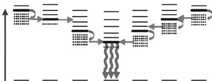
Figure 4.5 Exciton recycling in a LbL-assembled graded CdTe nanostructure. Excitons in the six layers of smaller-sized nanocrystals (NCs) may be trapped in surface states. However, the trapped excitons can be transferred very efficiently from layers with
