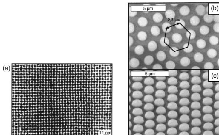
Figure 5.60 (a) TEM image of a 3-D aggregate consisting of 5.8 nm silver sulfide nanoparticles; (b) SEM image of superlattices of cobalt nanoparticles on HOPG; (c) Tilted SEM image
