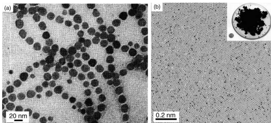
Figure 3.130 (a) Iron oxide nanocrystals synthesized from iron pentacarbonyl by Griffiths et al. in 1979. Reproduced with permission from Ref. [103]; © 1979, American Institute of Physics; (b) TEM image of monodisperse magnetite nanocrystals synthesized by
