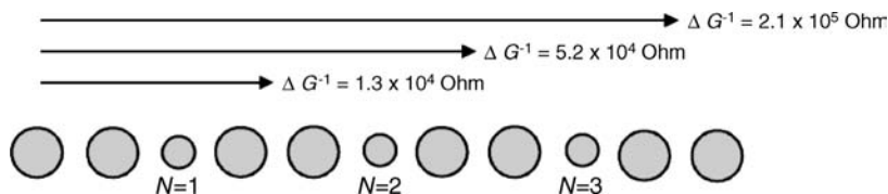
Figure 5.40 A 1-D chain of 2 nm metal particles with N = 3 “impurities” (i.e., 1 nm metal particles). The arrows indicate that the resistance increases exponentially with N [58].
