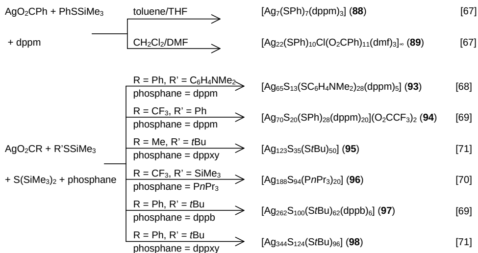
Scheme 3.10 Synthesis of various sulfur-bridged silver clusters by reactions of silver carboxylates with silylated sulfur compounds in the presence of tertiary phosphanes.
