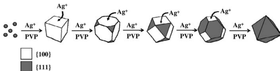
Figure 3.111 Shape evolution of polyhedral Ag nanocrystals.
