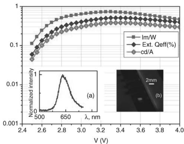
Figure 4.4 Efficiency values for a CdTe/PDDA light-emitting diode (LED). The device showed an electroluminescence turn on at 2.5 V, and maximum light output was obtained at 3.3 V and 350 \text{ mA cm}^{-2} , with a peak radiated power of 141 nW, corresponding to an external quantum efficiency of 0.51%. The luminous efficiencies
