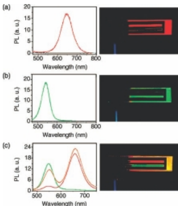
Figure 4.6 Photographs of lateral structures selectively formed by green- and red-luminescing CdTe nanocrystals via an electric field-directed LbL assembly, and the corresponding emission spectra. Reproduced with permission from Ref. [99].
