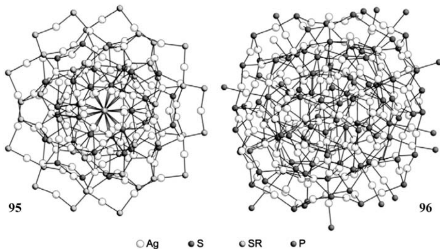
Figure 3.74 Molecular structures of [\text{Ag}_{123}\text{S}_{35}(\text{StBu})_{50}] ( 95 ) (left) and [\text{Ag}_{188}\text{S}_{94}(\text{PnPr}_3)_{20}] ( 96 ) (right).
