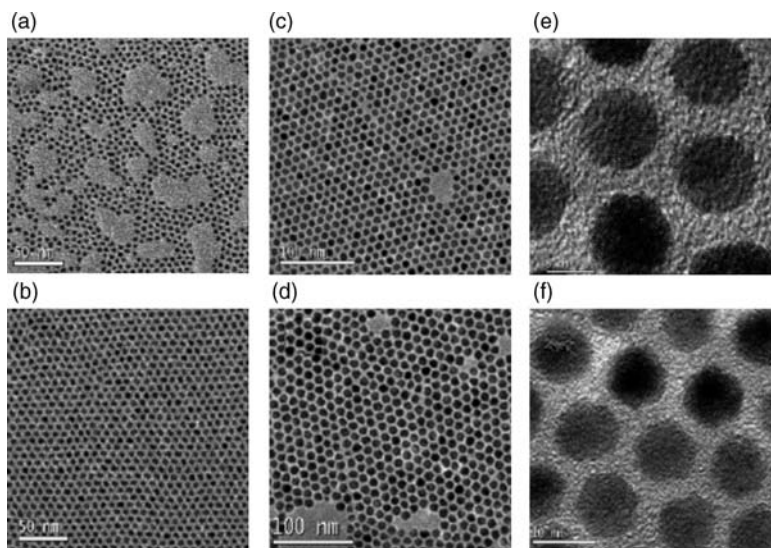
Figure 3.18 TEM images of the plain CdSe cores and core-shell nanocrystals obtained under typical reaction conditions. (a) TEM images of CdSe cores (before injection of \text{Cd}^{2+} solution); (b) (a) plus two monolayers of CdS; (c–e) (b) plus 3.5 monolayers of \text{Zn}_{0.5}\text{Cd}_{0.5}\text{S} ; (d–f) (c) plus two monolayers of ZnS. From Ref. [280].
