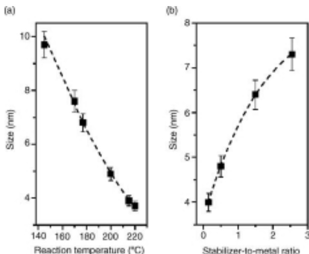
Figure 3.121 (a) Dependence of CoPt 3 nanocrystals size on the reaction temperature. (b) Influence of initial amount of the stabilizing agent (1-adamantancarboxylic acid) on nanocrystal size. Reproduced with permission from Ref. [55]; © 2003, American Chemical Society.
