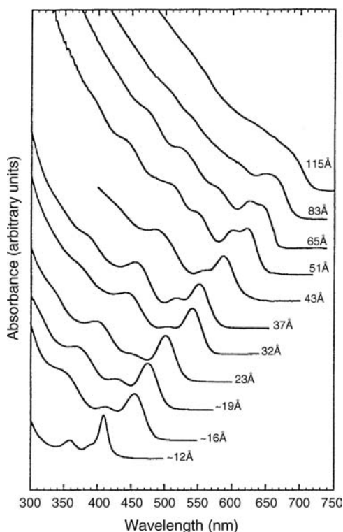
Figure 3.11 1993 state-of-the-art absorption spectra of CdSe colloidal solutions (“Hot-injection synthesis”). From Ref. [12].
