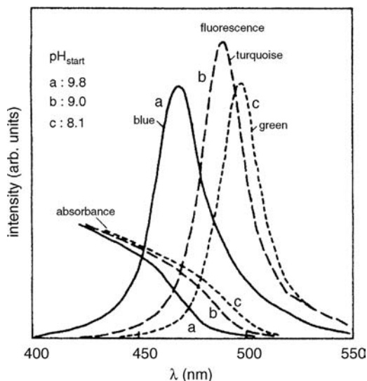
Figure 3.12 Absorption and luminescence spectra of \text{CdS} sols (“polyphosphate preparation”) with varying starting pH. From Ref. [28].
