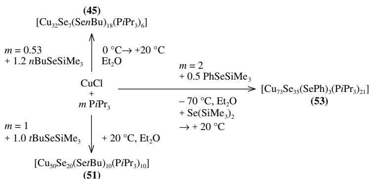
Scheme 3.7 Synthesis of various selenido–selenolato-bridged copper clusters in the presence of \text{PiPr}_3 under different reaction conditions.
