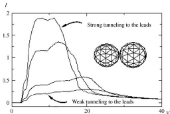
Figure 5.43 Increasing NDC effect for higher tunneling rates between array and reservoir in a two-nanoparticle array. Reproduced with kind permission from Ref. [59]; © 2005, American Physical Society.
