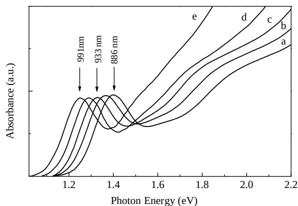
Figure 3.27 Evolution of the absorption spectra during the growth of InP shells on InAs cores with an initial radius of 1.3 nm (a). The InP shell thickness in number of monolayers is: (b) 0.5, (c) 1.1, (d) 1.7, (e) 2.5. Reproduced from Ref. [7].
