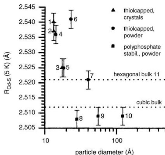
Figure 3.15 Mean Cd–S distances of thiol- and phosphate-stabilized CdS nanocrystals determined by extended X-ray absorption fine structure (EXAFS) spectroscopy at 5 K as a function of the particle diameter. From Ref. [163].
