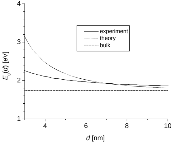
Figure 2.9 Size dependence of the energy gap E_g(d) for colloidal CdSe QDs with diameter d . The bulk value for the energy gap is E_g(\text{bulk}) = 1.74 \text{ eV} [60]. The theoretical curve was obtained using Eq. (2.17) with the following parameters: effective mass of electrons/holes m_e = 0.13 m_0 , m_h = 0.4 m_0 , m_0 = \text{mass of free electrons} ( m = 9.1095 \times 10^{-31} \text{ kg} ) \Rightarrow m^* = 0.098 m [60]; dielectric constant
