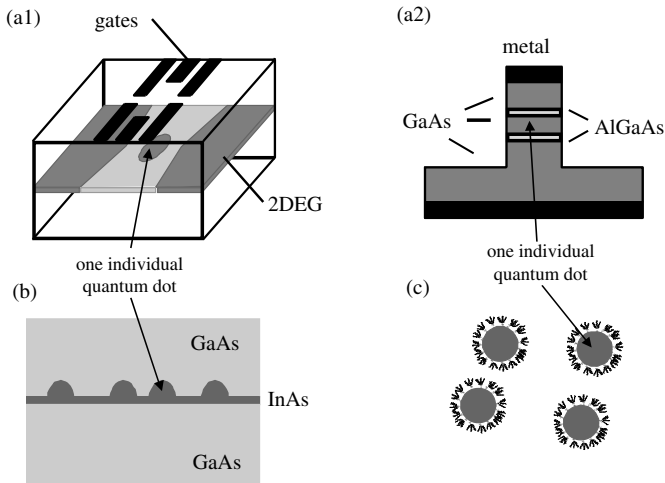
Figure 2.10 Three different types of quantum dot. (a1) A lithographically defined QD in lateral arrangement can be formed by electrostatic depletion of a 2-D electron gas (2DEG, shown in dark gray) via gate electrodes. The 2DEG is formed typically 20–100 nm below the surface of a semiconductor heterostructure (usually GaAs/AlGaAs). The application of negative voltages to metal gates on top of the heterostructure depletes the 2DEG below the gates (shown in light gray), and cuts out a small electron island from the 2DEG. Electrons can still tunnel onto and from the island. Electrical contact to the 2DEG is realized through Ohmic contacts (not shown); (a2) A vertical QD can be formed in a double-barrier heterostructure. A narrow pillar is etched out of a GaAs/AlGaAs/GaAs/AlGaAs/GaAs heterostructure. The AlGaAs layers (light gray) form tunnel barriers that isolate the central GaAs region from the
