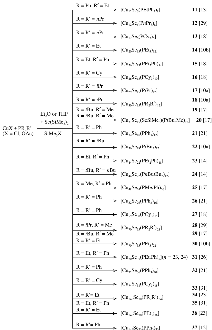
Scheme 3.4 Survey of the synthesis of selenium-bridged copper clusters protected by terminal phosphine ligands.
