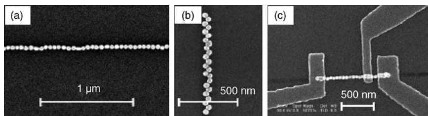
Figure 5.52 (a,b) Gold nanoparticle deposition along a patterned line with different widths; (c) Contacting the deposited nanoparticle chains by electron-beam lithography. Reprinted with permission from Ref. [67]; © 2008, American Institute of Physics.
