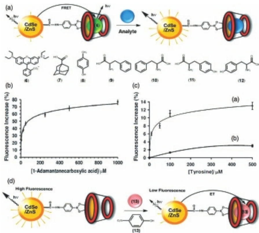
Figure 6.6 (a) Sensing of substrates by a competitive FRET assay using \beta -cyclodextrin-modified CdSe/ZnS QDs with receptor-bound rhodamine B ( 6 ); (b) Calibration curve corresponding to the analysis of variable concentrations of 7 by the rhodamine B/ \beta -cyclodextrin-modified CdSe/ZnS QDs system; (c) Calibration curve corresponding to
