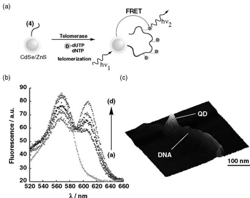
Figure 6.23 (a) Optical analysis of telomerase activity by the incorporation of Texas Red–dUTP into the telomeres associated with CdSe/ZnS QDs; (b) Time-dependent fluorescence changes upon telomerization of 31-functionalized QDs in the presence of telomerase extracted from 10 000 HeLa cells,
