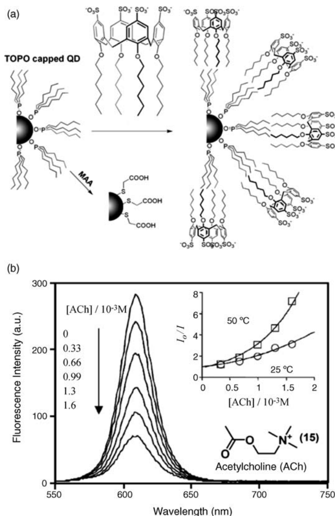
Figure 6.8 (a) Synthesis of TOPO-capped CdSe/ZnS QDs with tetrahexyl ether derivative of p -sulfonatocalix[4]arene receptor and MAA; (b) Quenching of the fluorescence emission of
