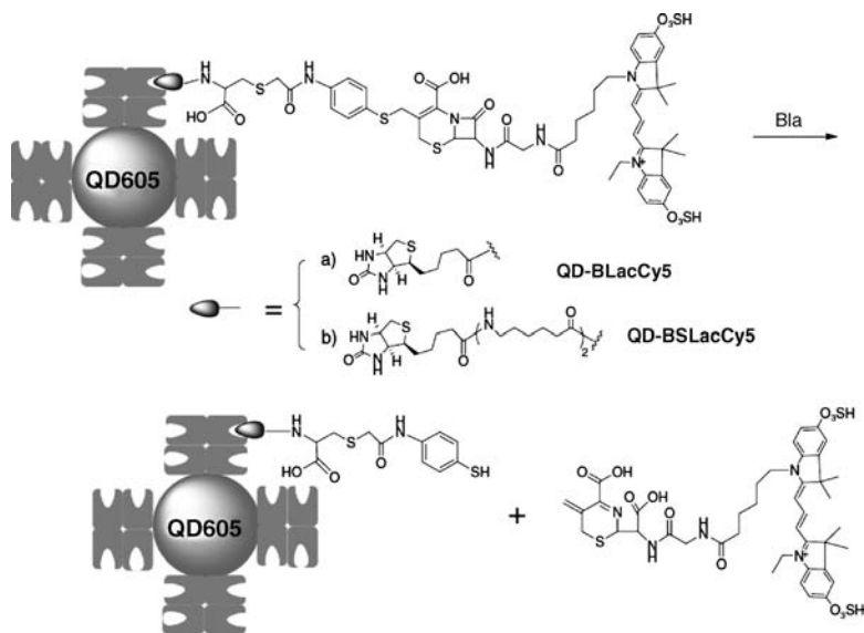
Figure 6.27 Optical detection of lactamase by modified-QDs. (Reproduced with permission from Ref. [193]).
