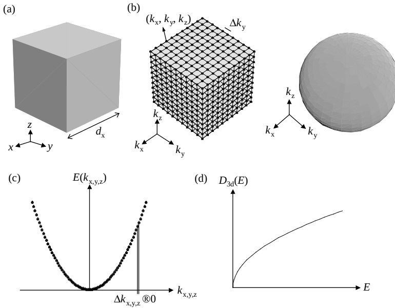
Figure 2.3 Electrons in a three-dimensional (3-D) bulk solid [16]. (a) Such a solid can be modeled as an infinite crystal along all three dimensions, x , y , and z ; (b) The assumption of periodic boundary conditions yields standing waves as solutions for the Schrödinger equation for free electrons. The associated wavenumbers (k_x, k_y, k_z) are periodically distributed in the reciprocal k -space [17]. Each of the dots shown in the figure represents a possible electronic state (k_x, k_y, k_z) . Each state in k -space can be only occupied by two electrons. In a large solid, the spacing \Delta k_{x,y,z} between individual electron states is very small and therefore the k -space is quasi-continuously filled with states. A sphere with radius k_F includes all states with k = (k_x^2 + k_y^2 + k_z^2)^{1/2} < k_F . In the ground
