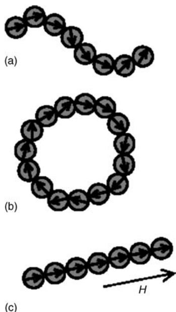
Figure 4.39 Dipolar chains formed by magnetic particles. (a) A semi-flexible chain of magnetic particles showing the head-to-tail, paired dipoles in the middle section and the unpaired dipoles at the ends; (b) A self-
