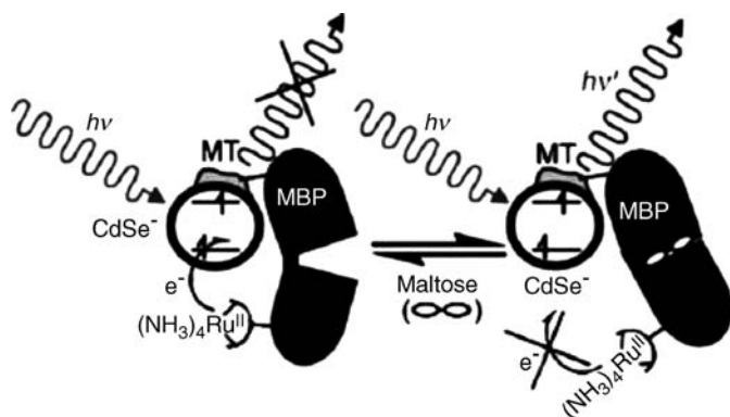
Figure 6.34 Controlling the degree of photoinduced electron transfer between CdSe and MBP functionalized with [\text{Ru}^{\text{II}}(\text{phenanthroline})(\text{NH}_3)_4] upon association
