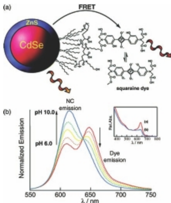
Figure 6.12 (a) Sensing of pH using the pH-sensitive squaraine dye conjugated to CdSe/ZnS QDs modified by an amphiphilic polymer associated with the hydrophobic nanocrystals; (b) Fluorescence spectra of the dye-modified
