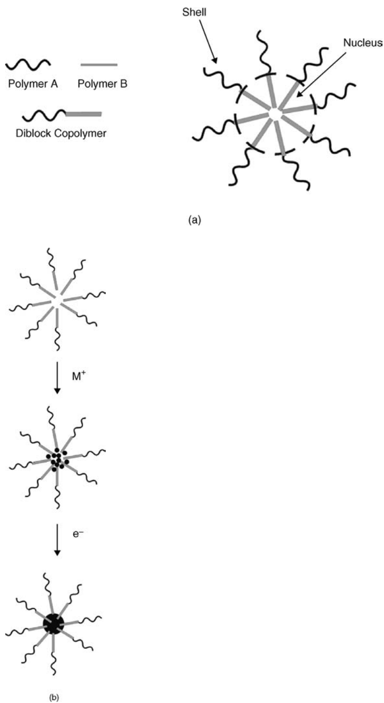
Figure 4.30 (a) Formation of diblock copolymers from polymer A and polymer B, resulting in micelles; (b) Formation of metal nanoparticles inside the micelles.
