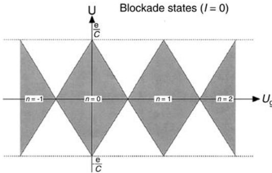
Figure 5.23 Idealized periodic rhomb pattern showing the Coulomb blockade region on the plane of voltages U and U_g . A transistor conducts only outside the rhombic-shaped regions. The value of the number n is the number of extra electrons trapped in the island in the blocked state.
