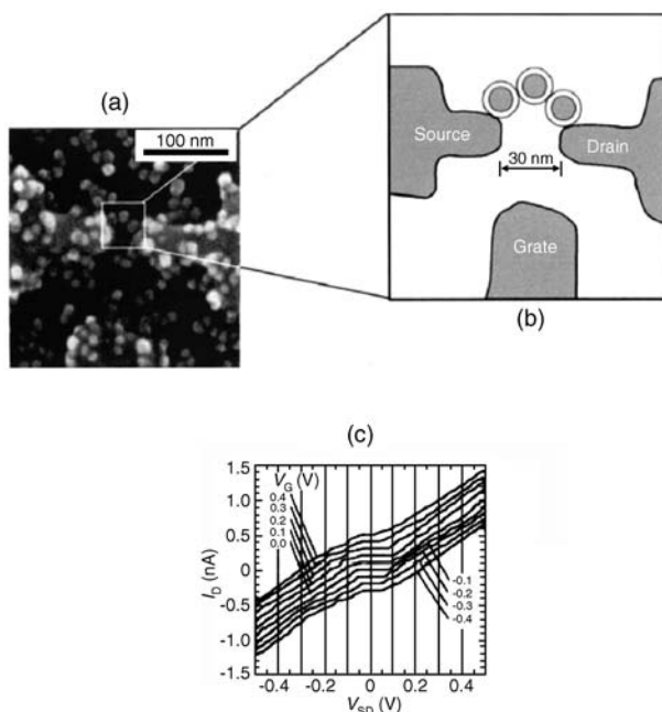
Figure 5.44 SET transistor, based on self-assembly of gold nanoparticles on electrodes fabricated by electron beam epitaxy. Reprinted with permission from Ref. [61]; © 1997, American Institute of Physics.
