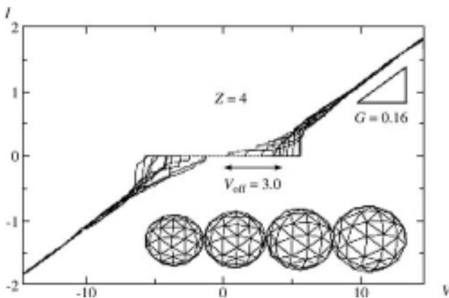
Figure 5.42 I(V) characteristics for different gate voltages of a four-nanoparticle array with growing diameter. Reproduced with kind permission from Ref. [59]; © 2005, American Physical Society.
