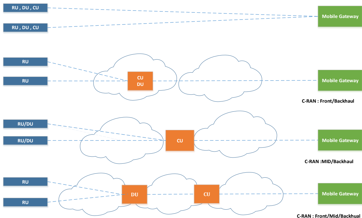
Figure 3-1 : RAN Architecture [16]
