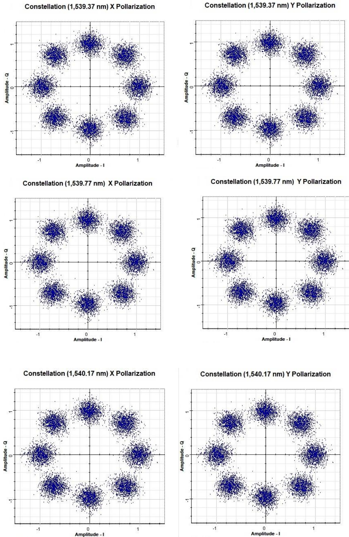
Figure 5-8 Constellation Diagram of Uplink signals for horizontal and vertical polarizations
