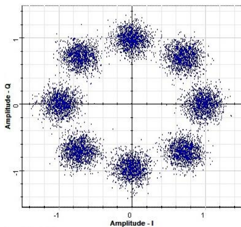
Constellation (1,560.57 nm) X Polarization
