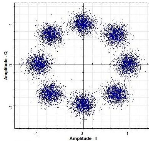
Constellation (1,560.17 nm) Y Polarization
