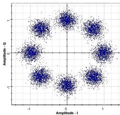
Constellation (1,560.57 nm) Y Polarization
