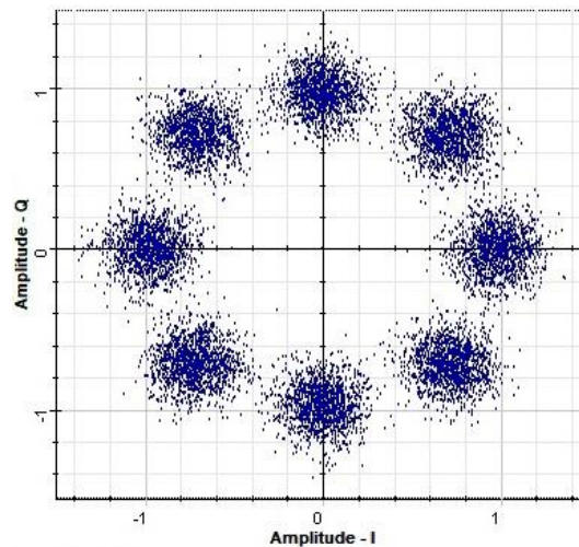
Constellation (1,559.77 nm) Y Polarization
