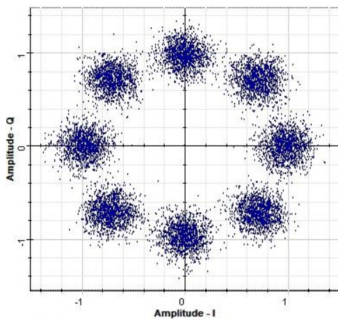
Constellation (1,559.77 nm) X Polarization
