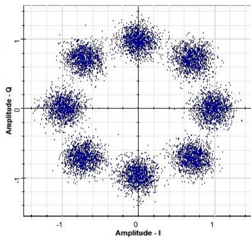
Constellation (1,560.17 nm) X Polarization
