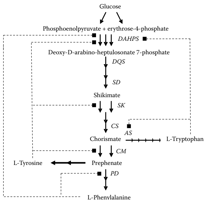
FIGURE 4.7 Biosynthetic pathways for L-tryptophan, L-phenylalanine, and L-tyrosine productions. Abbreviations for key enzymes are given in the text.
