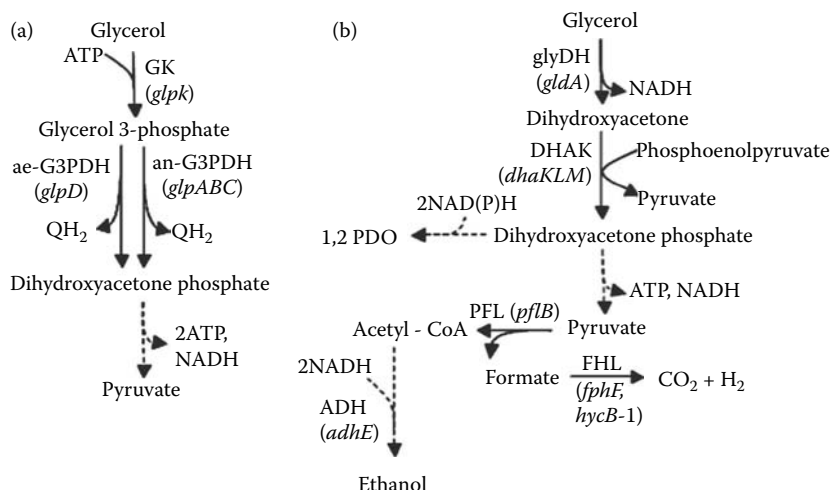
FIGURE 9.18 Anaerobic pathways for the co-utilization of glycerol and its conversion to pyruvate (a) and alcohol (b) by microorganisms. The glycerol pathway involves glycerol kinase (GK) and glycerol phosphate dehydrogenase (GPD) followed by glycolytic enzymes. (Durnin, G., et al. Biotechnology and Bioengineering , 103, 143–161, 2009.)
