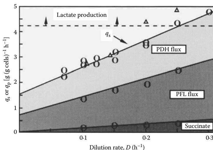
FIGURE 9.14 Specific sucrose consumption rate at 70 °C, pH 7.0. ( q_s = g. sucrose per g. cells per hour) for strain LLD-15 at 10 g. (O) and 15 g. (Δ) input sucrose per l. The hatched areas under the q_s line (arrowed) represent the proportion of the total pyruvate flux which goes via the PDH pathway, PFL pathway or to succinate. When q_s exceeds about 4.2 g sucrose (g cells) -1 h -1 , LLD-R revertants take over the cultures.
