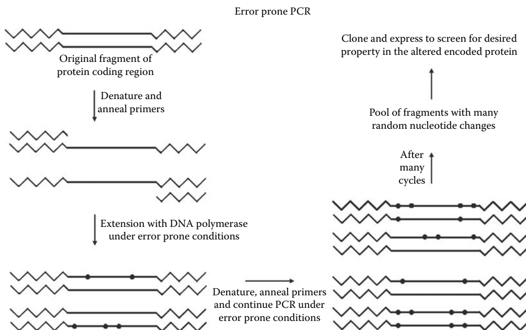
FIGURE 8.3 In error-prone PCR, the template is annealed with primers that allow for extension (by DNA polymerase) and incorporation of the dNTPs, deoxynucleotide triphosphates, in the incubation mixture. The condition of the extension and the enzyme used will define how frequently a mistake or misincorporation (e.g., A for G) is made. Denaturation of the strand at high temperature followed by reannealing of the primers can then allow the strands with mistakes to be copied, and the original strands and further errors by misincorporation are introduced, giving a product that may have many variations within the product molecules. Conditions can be used that will give an appropriate level of altered molecules (e.g., 1 mutation per 100 or 1000 residues on average). Because the molecules can be cloned and replicated independently within a plasmid, individual colonies with separate variants can again be isolated and screened for enzyme properties (e.g., high-temperature activity) and the specific DNA sequence of interesting variants can be analyzed.
