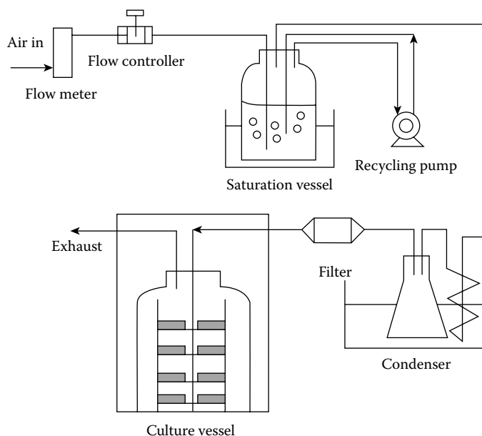
FIGURE 14.2 Shallow tray fermentor used for solid-state cultivation.
