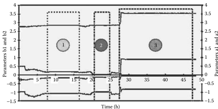
FIGURE 17.12 Estimation of system parameter.
