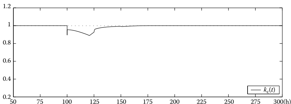
FIGURE 17.29 The system gain (with constraint of the controller parameter L(t) ).
