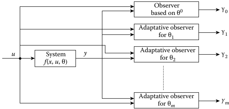
FIGURE 17.16 Bank of observers.
