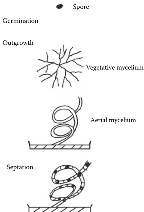
FIGURE 5.1 Diagram of the life cycle of Streptomyces .
