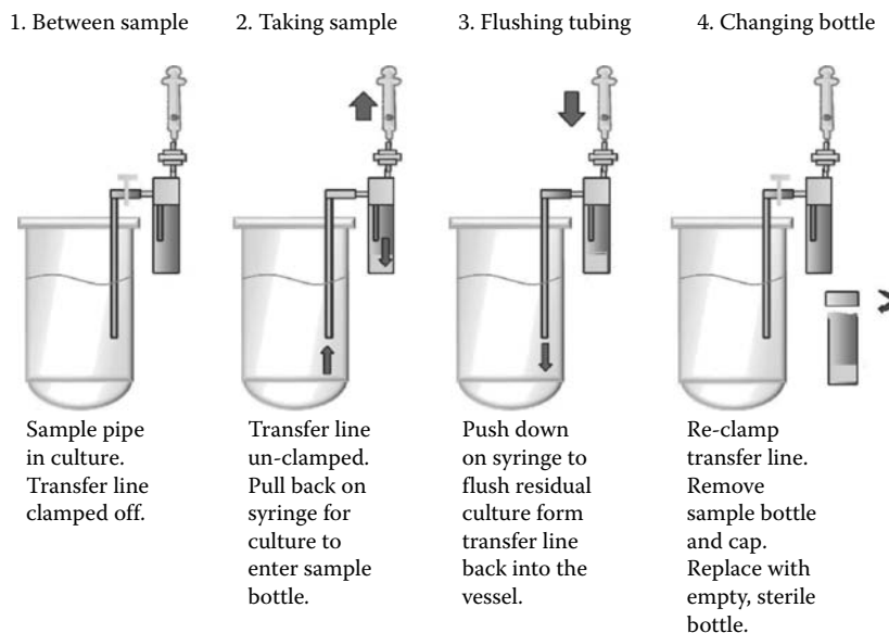
FIGURE 15.13 Sampling.
