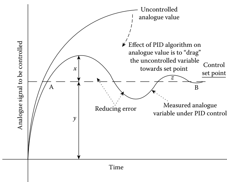
FIGURE 16.3 PID control.
