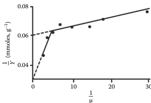
FIGURE 2.8 Graphical determination of maintenance ( m ) energy.
