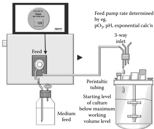
FIGURE 15.10 Feed control system.
