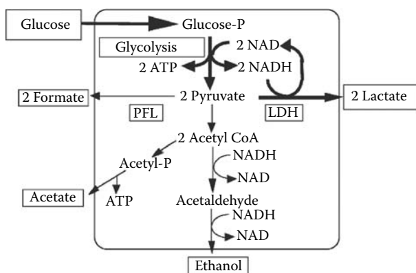
FIGURE 9.10 Anaerobic sugar metabolism in thermophilic Bacilli . The PFL growth pathway is on the left and the LDH overflow pathway is on the right.
